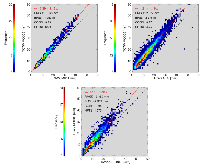
Figure 1. Normalized frequencies of occurrence for the comparison of the MODIS L2 TCWV product (MOD05) to ground-based microwave radiometers (3 sites: ARM SGP, TWP, NSA; left upper panel) and global ground-based GNSS data (right upper panel), both for the period 2003–2011, and AERONOT sun photometer measurements (lower panel) for the period 2003–2014. Figure 9 shows the geographical distribution of the validation data. See text for detailed information.
