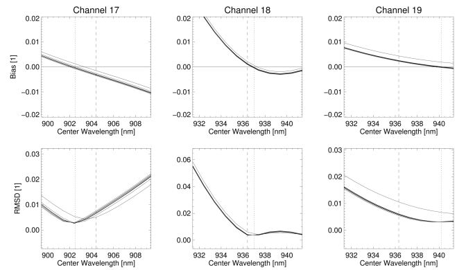
Figure 6. Assessment of the radiance–central wavelength dependency for MODIS Terra: bias (upper row) and RMSD (lower row) between simulated and measured radiances as a function of the assumed central wavelength for each absorption band. Each curve represents 1 of the 10 detectors. The vertical dashed lines indicate the position of the original nominal wavelength of the band. The vertical dotted lines indicate the position of zero bias and minimum RMSD. See text for further discussion (Sect. 4).
