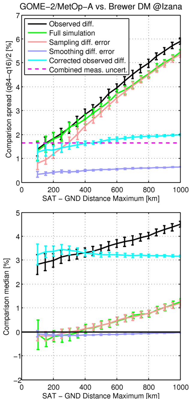
Figure 11. Upper panel: observed and simulated comparison spread between GOME-2/MetOp-A TOC measurements and correlative Brewer observations as a function of maximum co-location distance for the Izaña station over the period 2007–2010. Lower panel: comparison median for the same sets of comparisons. Colours as in the upper panel.
