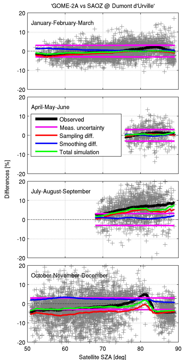
Figure 8. SZA dependence of the differences between GOME-2A and the SAOZ at Dumont d'Urville, grouped per season and covering 2007 to 2009. Grey crosses denote individual observed differences and solid lines represent the running 5^\circ SZA median. While not perfect, the simulations qualitatively reproduce the observed SZA dependence, e.g. the increasing median in local winter, and the feature at 80^\circ SZA in local spring.
