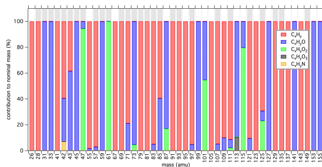
Figure 10. PTR-TOF mass contributions for all the masses that showed ambient signal during UBWOS2013. The grey bars on top indicate the masses that were monitored with the PTR-QMS.
