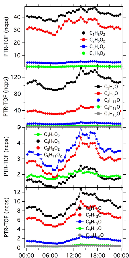
Figure 11. PTR-TOF diurnal variation of selected oxygenated VOCs during UBWOS2013. Many of those compounds cannot be unambiguously identified with PTR-QMS.
