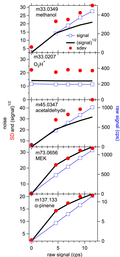
Figure 5. Signal, (\text{signal})^{1/2} , and standard deviation (SD) of the signal (noise) during a typical PTR-TOF calibration measurement for some selected masses.
