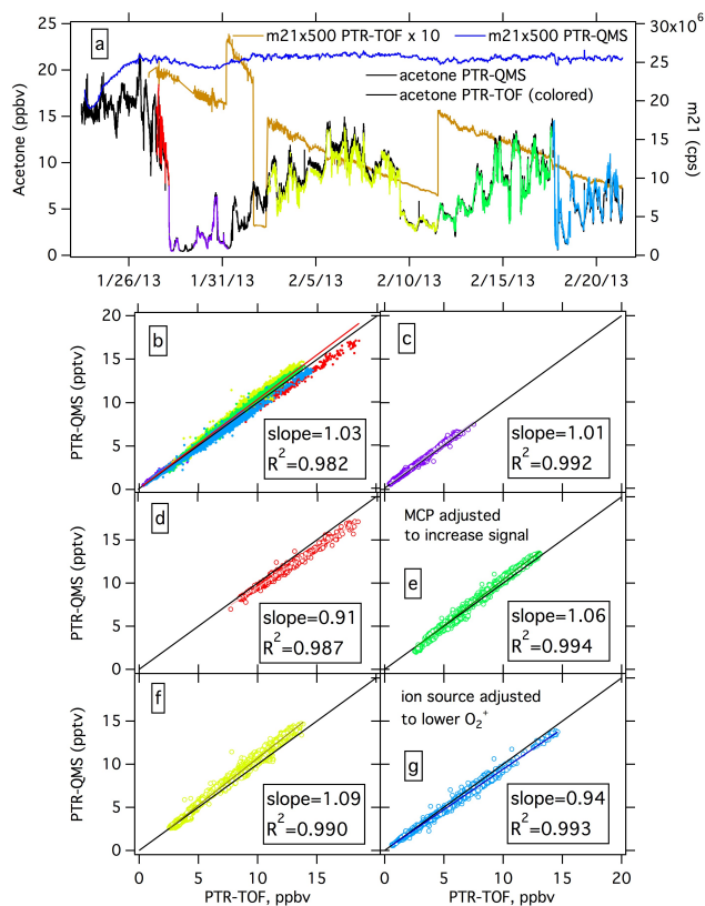
Figure 7. PTR-QMS and PTR-TOF acetone intercomparison during UBWOS2013: (a) time series of the PTR-TOF and PTR-QMS primary ions and acetone. The color code of the PTR-TOF acetone signal indicates when the PTR-TOF was relatively stable. (b) Scatter plot of PTR-QMS and PTR-TOF acetone for the whole campaign. (c–g) Scatter plots for separate stable periods of the PTR-TOF.
