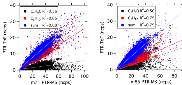
Figure 8. PTR-QMS and PTR-TOF intercomparison for mass 71 and mass 85 during UBWOS2013.
