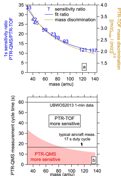
Figure 4. (a) The ratio of the 1 s sensitivities of PTR-QMS / PTR-TOF together with the PTR-TOF mass discrimination. (b) A mass-dependent curve showing the length of the PTR-QMS measurement cycle, where the PTR-QMS is as sensitive as the PTR-TOF (identical to the fit in a). In aircraft measurements a duty cycle of 17 s is typical (PTR-TOF more sensitive above mass 80) and at ground sites 1 min measurements are typical (PTR-TOF more sensitive for all masses).
