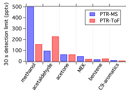
Figure 6. PTR-QMS and PTR-TOF 30 s detection limits during UBWOS2013.
