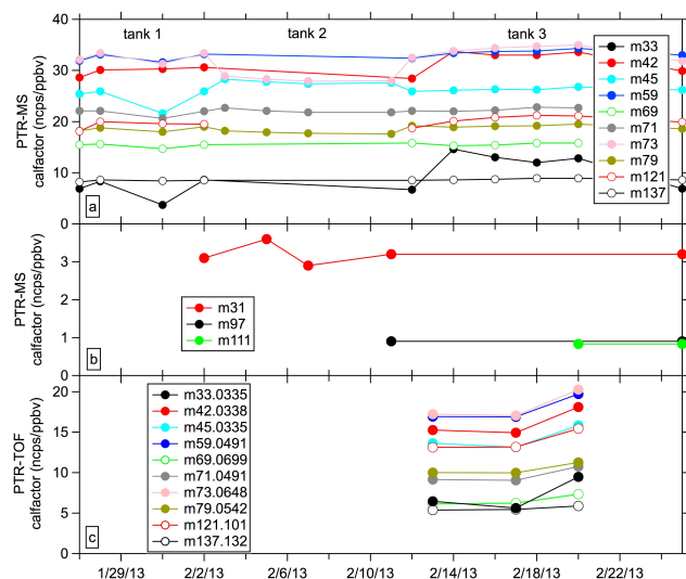
Figure 2. (a) Multiple VOC PTR-QMS calibration using three different calibration gas tanks during UBWOS2013: methanol (m33), acetonitrile (m42), acetaldehyde (m45), acetone (m59) isoprene (m69), methacrolein (m71), methylethylketone (m73), benzene (m79), 1,3,5-trimethylbenzene (m121) and \alpha -pinene (m137). (b) PTR-QMS calibrations using the MOCCS cart for formaldehyde (m31), methylcyclohexane (m97) and dimethylcyclohexane (m111). (c) PTR-TOF calibration for the same compounds as in (a) during UBWOS2013.
