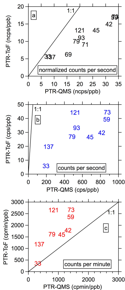
Figure 3. (a) PTR-QMS and PTR-TOF sensitivity in \text{ncps ppbv}^{-1} normalized to 1 \times 10^6 \text{ H}_3\text{O}^+ ions. (b) Sensitivity in \text{cps ppbv}^{-1} with PTR-QMS 25 \times 10^6 and PTR-TOF 1.6 \times 10^6 \text{ H}_3\text{O}^+ ions. (c) Sensitivity in \text{cpmin ppbv}^{-1} with PTR-QMS measuring 37 ions. The numbers in (a), (b) and (c) are the nominal mass of the calibrated compounds.
