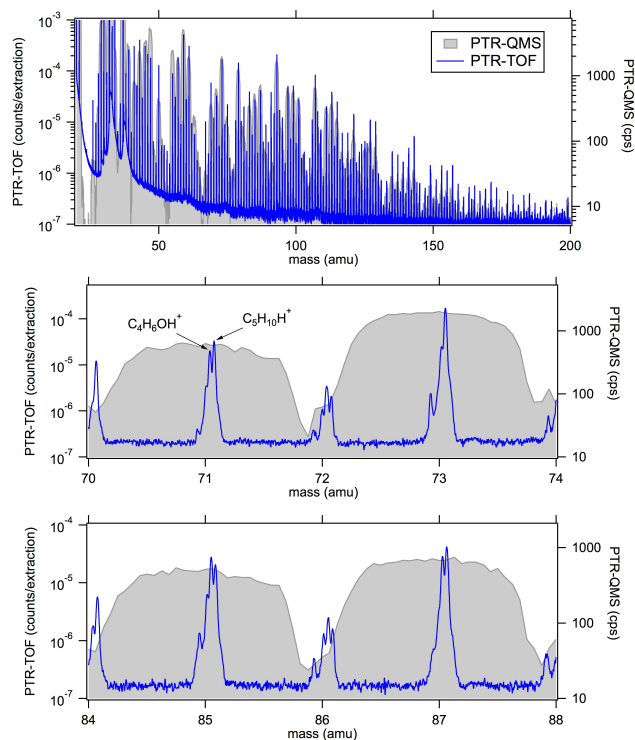
Figure 9. PTR-QMS and PTR-TOF mass scans. As an example, for m/z 71 two isobars are identified with the PTR-TOF and labeled.
