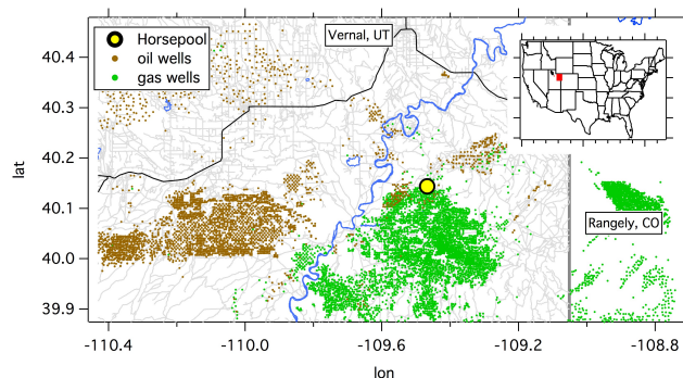
Figure 1. Map of the study area with the Horse Pool ground site in the Uintah Basin, Utah.
