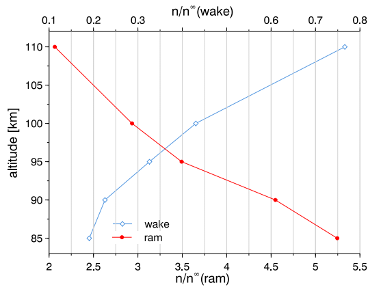
Figure 10. Ratios between local and free-stream total number density at the sensor position as a function of altitude. The ratios are obtained from numerical simulations made at the marked altitudes and are used as aerodynamic correction factors.
