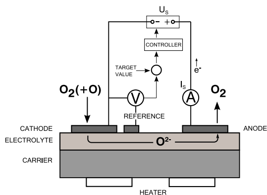
Figure 2. Electrical circuit of a sensor with three-electrode design and regulation of the reference voltage.
