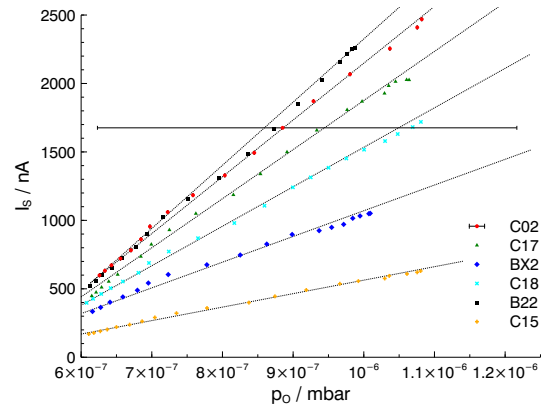
Figure 6. Calibration curves for the atomic oxygen sensors labeled C02–C15 flown on WADIS-1. Sensor currents are plotted over atomic oxygen partial pressure. The error bar represents the uncertainty due to the pressure measurement and shifted electron energy in the QMS ionizer.
