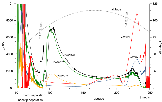
Figure 8. Raw signals of the atomic oxygen sensors vs. flight time, together with the altitude and rocket orientation during the experimentation phase.
