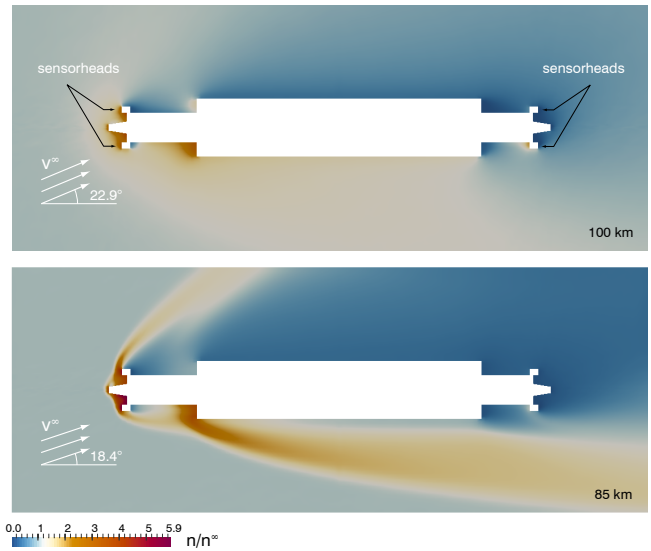
Figure 9. Distribution of the ratio between local and free-stream number density during the downleg at two different altitudes. Results from 3D DSMC calculations with the PICLas code.
