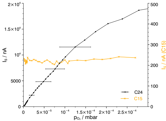
Figure 7. Calibration curves for molecular oxygen sensor C24 with platinum electrodes and for atomic oxygen sensor C15 with gold-plated cathode. Sensor currents are plotted over the O 2 partial pressure. The error bars indicate the uncertainty due to the pressure measurement.
