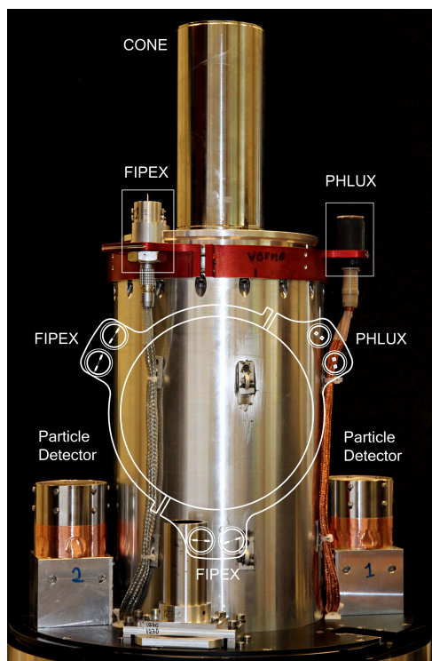
Figure 4. Payload on the fore deck of the rocket with both a FIPEX and PHLUX sensor head visible and a sketch showing their arrangement. Other instruments in the photo are the particle detectors and the CONE ionization gauge, all from IAP. CONE is covered by an evacuated hood.
