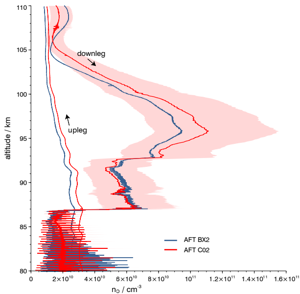
Figure 12. Measurement results for atomic oxygen number density vs. altitude for sensors on the aft deck during the up- and downleg without aerodynamic correction. The shading shows the uncertainty from the calibration for the aft sensor CO 2 .
