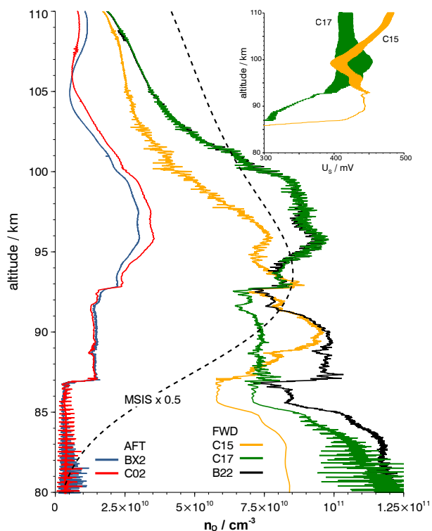
Figure 16. Comparison of O number density profiles from sensors on fore and aft deck during the downleg after aerodynamic correction (ram factors for aft, wake factors for fore). The MSIS profile is scaled by 0.5 and plotted additionally. The inset shows the course of the sensor voltage U_S (including 2.9 Hz modulation from rocket spin) for two fore sensors.
