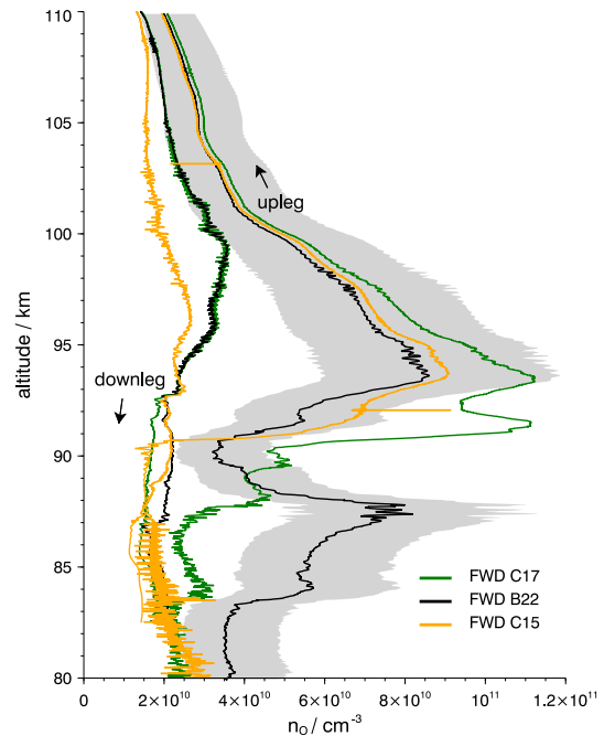
Figure 11. Measurement results for atomic oxygen number density vs. altitude for sensors on the fore deck during the up- and downleg without aerodynamic correction. The shading shows the uncertainty from the calibration for fore sensor B22.
