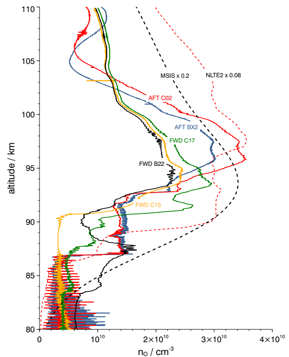
Figure 14. Profiles of O number density for FIPEX sensors on fore and aft deck after aerodynamic ram correction. Downleg profile for aft sensors, upleg part for the fore sensors. Comparison to MSIS model and NLTE-2 measurements.
