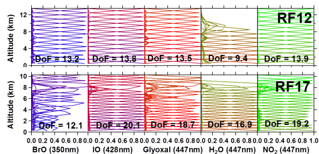
Figure 7. Characterization of the AMAX profiles of BrO, IO, glyoxal, H 2 O and NO 2 in terms of AVK and DoF for RF12 and RF17. The larger number of DoF during RF17 is the result of a shorter integration time for limb spectra during the aircraft ascent. See Sects. 2.8 and 3.3.
