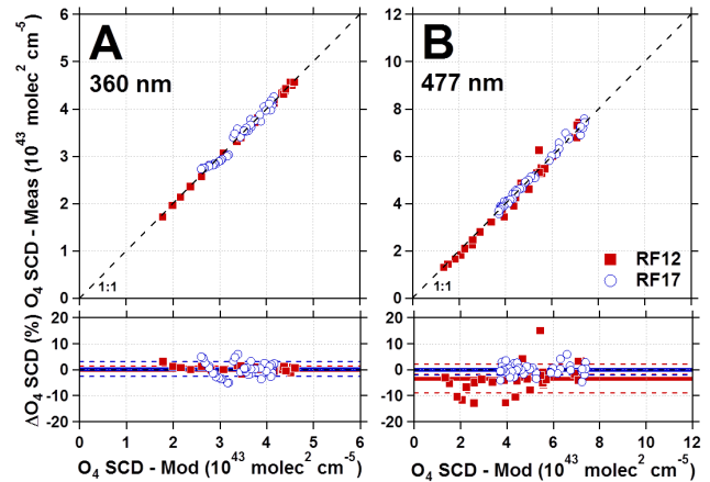
Figure 4. Comparison of measured and predicted O_4 SCDs for the two profile case studies. The lower panels show the relative difference to the 1 : 1 line; solid lines represent the median bias and dashed lines the 1\sigma standard deviation of scatter around the 1 : 1 line.
