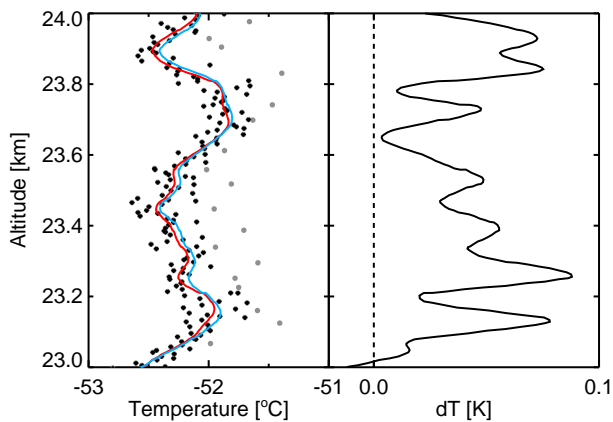
Figure 8. Left panel: temperature profile before (black dots) and after smoothing and consecutive spike removal (red trace). The grey dots represent the temperature spikes that were removed by the spike-removal algorithm. The blue trace represent the smoothed profile before spike removal. The right panel shows the difference between the blue and the red curves. The sounding was performed in Lindenberg on 16 August 2012 (12:00 UTC); maximum solar zenith angle during the sounding: 48.9^\circ .
