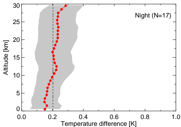
Figure 10. Uncertainty of the temperature measurements, determined from 29 noon (top) and 17 midnight (bottom) RS92 dual launches performed in Lindenberg. The red line represents the mean of the difference of GRUAN temperature profiles; the black trace denotes the estimated uncertainty profile calculated for soundings performed on 17 September 2013; both traces are given for k = 2 . The grey band represents the standard deviation of the measured temperature differences. Data are gridded in 1 km wide bins. The maximum solar zenith angle during the noon sounding was 36.5^\circ .
