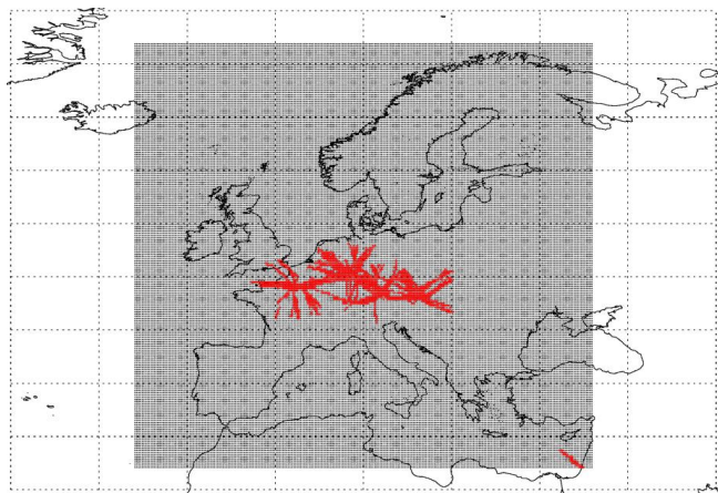
Figure 5. MOCAGE regional chemistry-transport model domain and corresponding MOZAIC/IAGOS profile measurements (flights paths; red) that were made during the two periods for which the MOCAGE simulations were available (June 2003–August 2003 and November 2003–January 2004).
