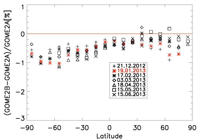
Figure 6. Latitudinal average differences (collocated data) of total ozone columns from GOME-2A and GOME-2B for 21 December 2012, 19 January, 17 February, 3 March, 18 April, 15 May and 15 June 2013.
