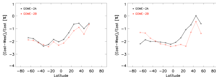
Figure 3. The scan angle dependency of ozone vertical column densities as function of latitude for GOME-2A (2008, black) and GOME-2B (2013, red) for January (left) and June (right). East pixels represent scan angles smaller than 0^\circ and west pixels represent scan angles larger than 0^\circ .
