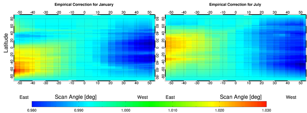
Figure 4. Empirical correction factors as a function of latitude and scan angle (East: scan angle < 0^\circ ; West: scan angle > 0^\circ ) for January and July. Correction ratios larger than one (red) are mostly found for the eastern part of the scan, while correction factors smaller than one (blue) correspond mostly to the western part of the scan.
