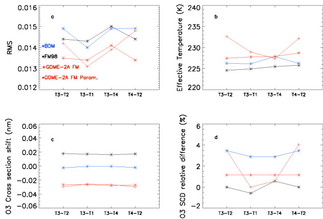
Figure 1. (a) RMS fit residuals, (b) effective temperatures, (c) O_3 cross-section wavelength shifts, and (d) the change in O_3 slant column relative to the column obtained using GOME FM98 cross sections at 241 and 221 K (GDP 4.4 settings), obtained after DOAS retrieval of the pixel 8500 of the GOME-2A orbit 20392, using different combinations of O_3 absorption cross-section data sets. For the GOME FM98 data set, T1, T2, T3 and T4 represent 202, 221, 241 and 273 K respectively. For the GOME-2A FM data set, T1, T2, T3 and T4 represent 203, 223, 243 and 273 K respectively. For the BDM data set, T1, T2, T3 and T4 represent 218, 228, 243 and 273 K respectively.
