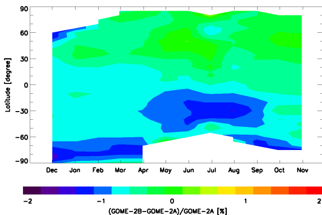
Figure 8. Time series of the zonally mean difference between GOME-2A and GOME-2B total ozone columns from December 2012 to November 2013.
