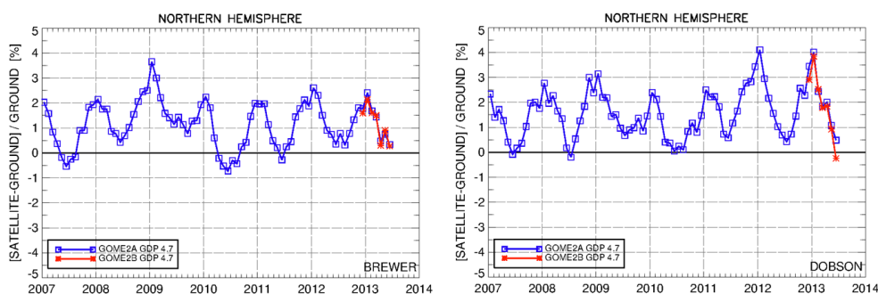
Figure 13. Time series of the monthly mean percentage differences between GOME-2A GDP 4.7 (blue line) and GOME-2B GDP 4.7 (red line) against the Northern Hemisphere Brewer stations (left panel) and the Northern Hemisphere Dobson stations (right panel).
