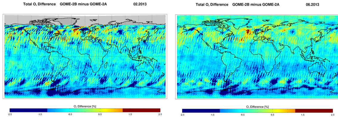
Figure 7. Monthly average differences between total ozone columns from GOME-2A and GOME-2B for February (left) and June 2013 (right).
