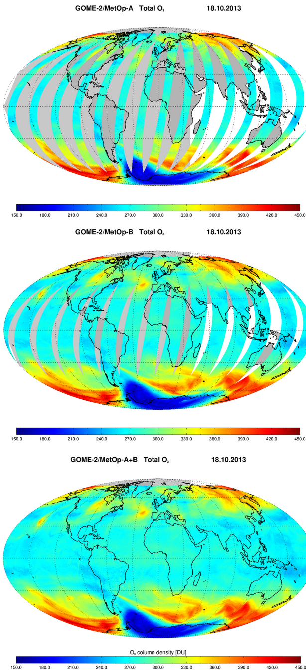
Figure 11. Total ozone column retrieved only from GOME-2A (top) and GOME-2B (middle), and GOME-2A and 2B (bottom) on 18 October 2013.
