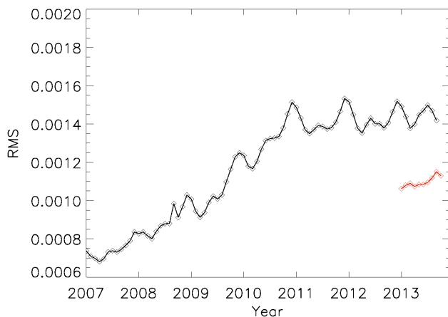
Figure 5. Long-term DOAS fitting residuals for the 325–335 nm ozone fitting window for GOME-2A (black line) and GOME-2B (red line). The monthly averaged residual values have been calculated for the equatorial Pacific region ( 10^\circ S– 10^\circ N, 160^\circ E– 160^\circ W).
