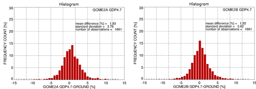
Figure 14. Histogram representation of the daily relative differences between GOME-2A GDP 4.7 (left panel) and GOME-2B GDP 4.7 (right panel) against the global Dobson station network in the period December 2012 to June 2013.
