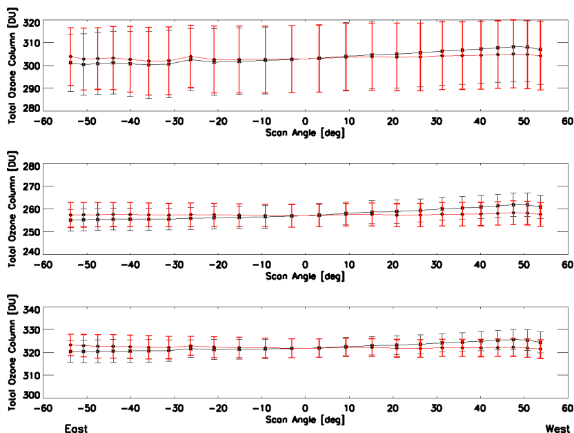
Figure 10. Dependency of GOME-2B total ozone column on instrument scan angle (forward scan only) without (black) and with (red) the empirical scan angle correction for all latitudes (top), tropics (middle) and midlatitudes (bottom).
