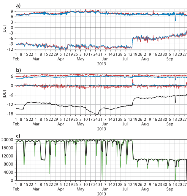
Figure 15. The top plots show the time series from 1 February to 30 September 2013 of first-guess (red) and analysis (blue) departures (dotted lines) and their standard deviations (solid lines) of GOME-2 total column ozone from the MACC NRT analysis which included the data passively; the middle plot shows the same for an experiment in which the GOME-2 TOC data were assimilated. The black line in the middle panel shows the bias correction applied to the data, and the bottom panel shows the number of observations used in this experiment.
