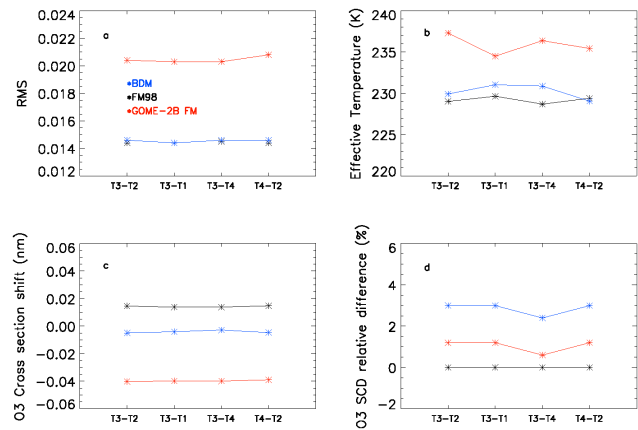
Figure 2. (a) RMS fit residuals, (b) effective temperatures, (c) O_3 cross-section wavelength shifts, and (d) the change in O_3 slant column relative to the column obtained using GOME FM98 cross sections at 241 and 221 K (GDP 4.4 settings), obtained after DOAS retrieval of the pixel 5144 of the GOME-2B orbit 5392, using different combinations of O_3 absorption cross-section data sets. The meanings of T1, T2, T3 and T4 are the same as in Fig. 1.
