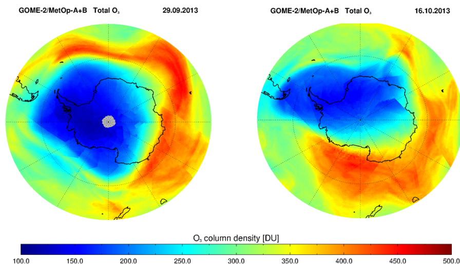
Figure 12. Total ozone maps for 29 September and 16 October 2013 based on data from GOME-2A and GOME-2B.
