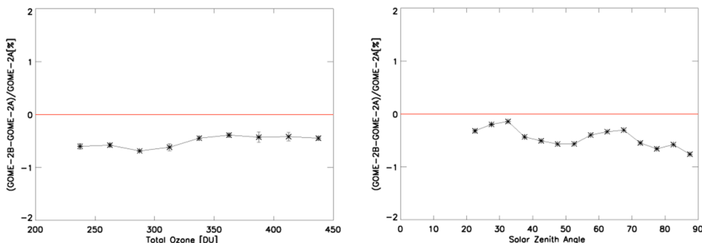
Figure 9. Relative difference between GOME-2A and GOME-2B total ozone columns as a function of total ozone column (left) and solar zenith angle (right). One year (from December 2012 to November 2013) of GOME-2A and GOME-2B data are used.
