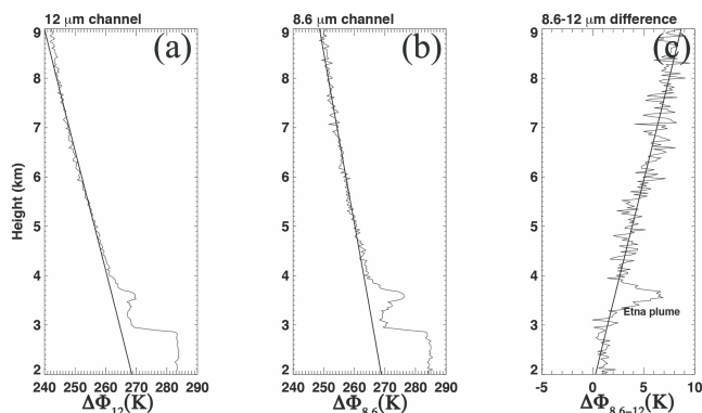
Figure 7. (a) Brightness temperature versus height variation for the 12 \mu\text{m} filter ( \Phi_{12} ). (b) Brightness temperature versus height variation for the 8.6 \mu\text{m} filter ( \Phi_{8.6} ). (c) Brightness temperature difference versus height variation for the 8.6–12 \mu\text{m} filters ( \Delta\Phi_{8.6,12} ). The straight lines are least-squares linear fits based on profile data above the plume, and extrapolated through and below the plume.
