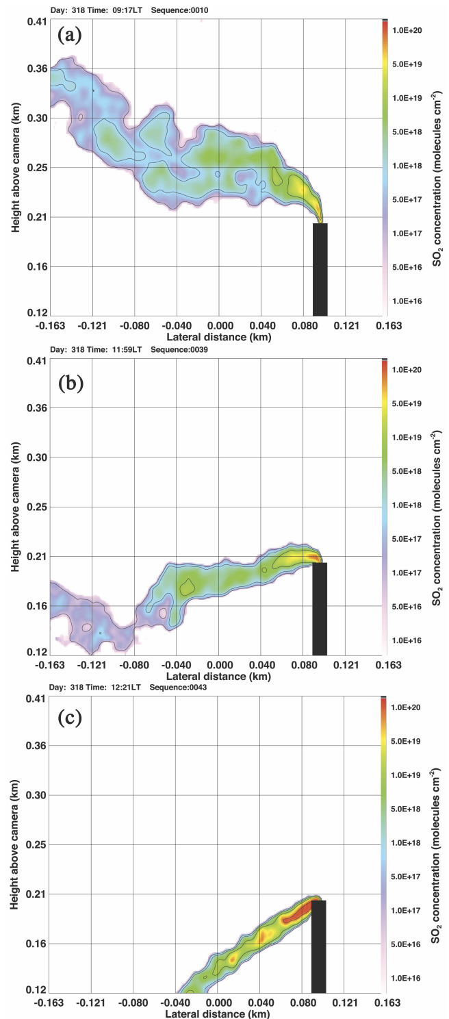
Figure 14. Cyclops measurements of the \text{SO}_2 plume from the industrial stack at the Port Pirie lead smelter, showing different behaviours of the plume. (a) Lofted plume, (b) fumigation and (c) grounding.
