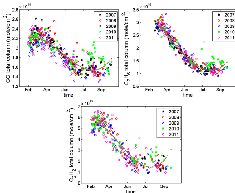
Figure 10. Daily mean total columns (in molecules \text{cm}^{-2} ) of CO, HCN and C 2 H 6 , plotted in different colours for the different years of measurements. The brown lines show the polynomial fits to the data.
