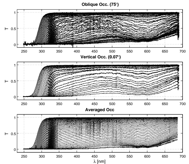
Fig. 1. Example of GOMOS transmittance spectra for an oblique occultation (top panel), a vertical occultation (middle panel) and an averaged occultation (bottom panel). The altitude range is 15–60 km.
