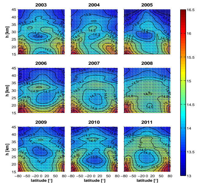
Fig. 7. Latitude–altitude maps of OCIO slant column densities (log scale, \text{cm}^{-2} ) retrieved from GOMOS measurements for years 2003–2011. Latitude range of 80^\circ \text{ S} – 80^\circ \text{ N} , altitude range of 15–45 km.
