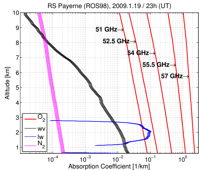
Fig. 5. Absorption Coefficient versus altitude for oxygen (O 2 ), water vapor (ww), liquid water (lw) and nitrogen (N 2 ) at 51, 52.5, 54, 55.5 and 57 GHz calculated with radiosonde data from Payerne on 19 January 2009 (I WV = 13.11 mm, I LW = 0.19 mm). Calculations made with the Rosenkranz (1998) model.
