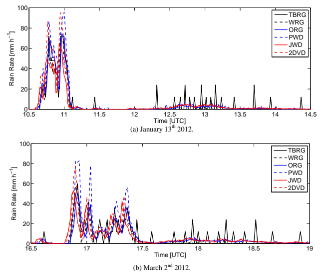
Fig. 3. Evolution of the rain rate recorded by six instruments.
