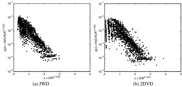
Fig. 8. Experimental scattergram of the general function from JWD and 2DVD.
