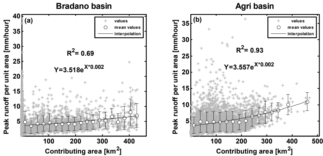
Fig. 6. Mean value of the peak runoff per unit area at the event scale as a function of contributing area for semi-arid basin (a) and sub-humid basin (b).
