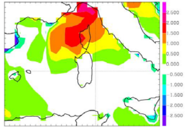
Fig. 8. SST difference (K) between ECMWF and ARPEGE analyses for 13 September 2006.
