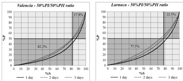
Fig. 10. Precipitation % & rain-spells % relationship for RSD=1, 2, 3 days.
