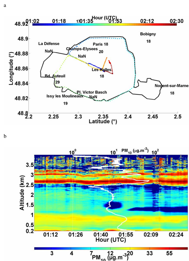
Fig. 9. Route followed by the small vehicle embarking the lidar on the 27 May 2005 over the Paris ring (a), and corresponding 2-D colour-coded temporal evolution of lidar-derived PM 10 concentrations (b). Hourly averaged PM 10 values measured by AIRPARIF network stations are reported in panel (a). The mean PM 10 profile retrieved from lidar signals is shown in white in panel (b). The black line circling Paris on the map (a) is the geographic demarcation of Paris city.
