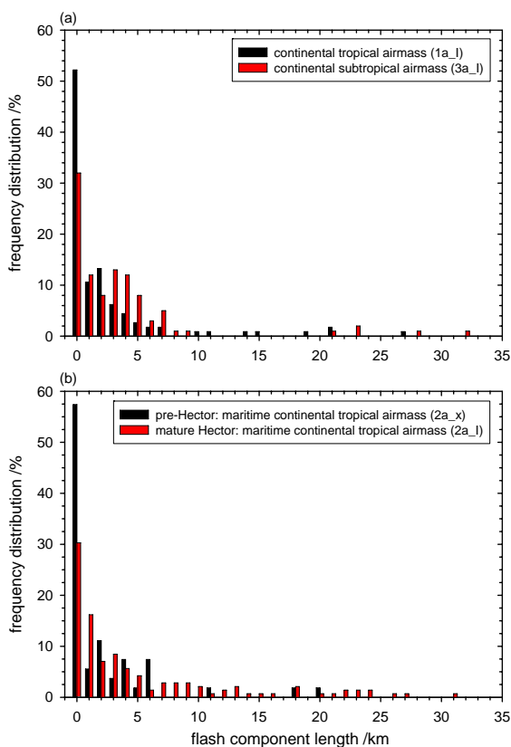
Fig. 18. Frequency distributions of LINET flash component lengths on 19 November 2005 for thunderstorm “1a.I” and “3a.I” (a) and for thunderstorm “2a.x” and “2a.I” (b). For a given flash component length of e.g. “1 km”, all lengths between \geq 1.0 and < 2.0 km were summarised.
