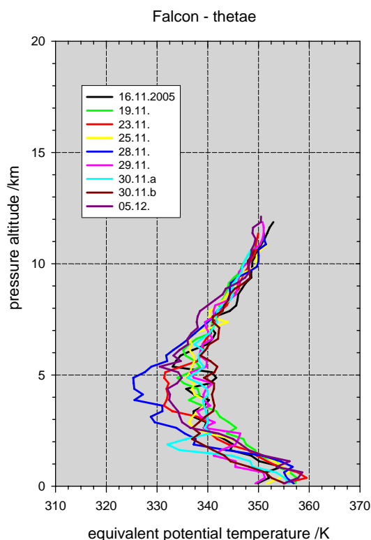
Fig. 14. Mean vertical profiles for the equivalent potential temperature ( \Theta_e ) derived from measurements with the Falcon aircraft. Mean values for every 250 m altitude bin are given for all available SCOUT-O3 flights (dd:mm:(yyyy)) in colour.
