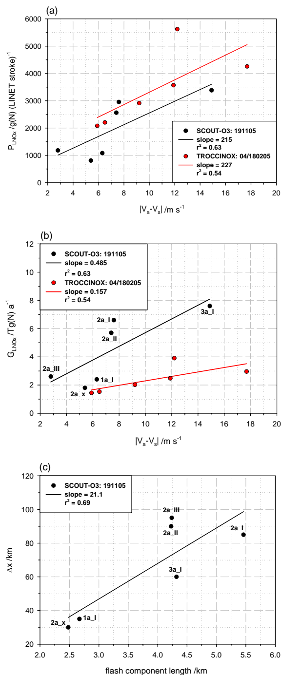
Fig. 17. Correlation between the vertical wind shear v_a - v_s (between the anvil outflow and the steering level) and the LNO x production rates P_{LNO_x} (a) and G_{LNO_x} (b) for selected SCOUT-O3 and TROCCINOX thunderstorms (labelled in (b) and (c)). Different LINET/LIS factors were used in (b): 1.6 for SCOUT-O3 and 0.5 for TROCCINOX. In (c) the correlation between the flash component length and the width \Delta x of the anvil outflow perpendicular to the wind direction is shown.
