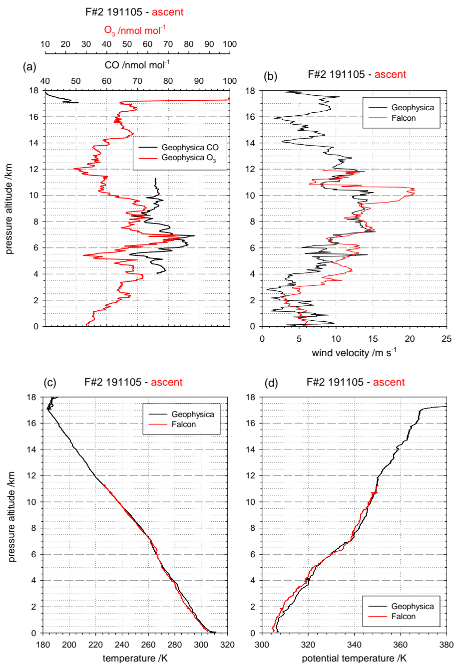
Fig. 11. Vertical profiles for CO and O 3 (a), wind velocity (b), temperature (c), and potential temperature (d) derived from measurements with the Falcon and Geophysica aircraft during ascent on 19 November 2005.
