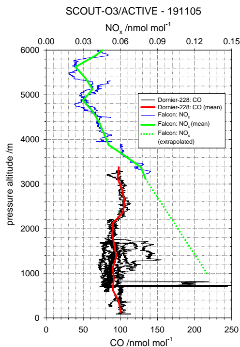
Fig. 10. Vertical NO x and CO profiles derived from measurements with the Falcon and Dornier-228 aircraft on 19 November 2005. Mean values are given for every 250 m altitude bin (bold lines). An extrapolation of the measured NO x mixing ratios down to 1 km is indicated by the dotted line.
