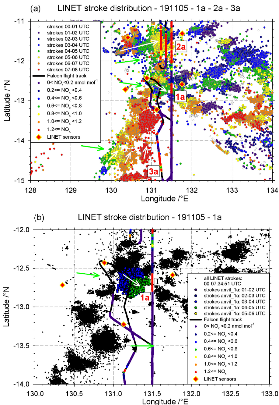
Fig. 7. Spatial and temporal LINET stroke distribution on 19 November 2005 between 00:00 and 08:00 UTC (upper colour scale). The observed NO x mixing ratio along the Falcon flight path is superimposed (lower colour scale). Enhanced NO x mixing ratios were observed during the passage of the anvil outflow of thunderstorms with lightning activity labelled “1a”, “2a”, and “3a” in (a). All strokes registered before the Falcon penetrated the selected thunderstorm systems “1a”, “2a”, and “3a” are coloured in (b), (c), and (d), respectively. The white arrows indicate the direction of the storm motion and the green arrows the main wind direction in the anvil outflow (not scaled according to velocity). In addition, the positions of the LINET sensors are indicated (diamonds).
