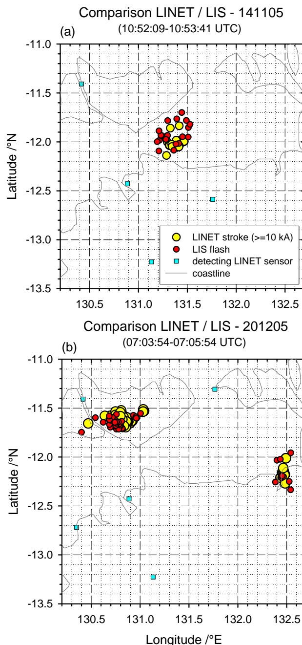
Fig. 15. Horizontal distributions of LIS flashes (in red) and LINET strokes with peak currents \geq 10 kA (in yellow) during the LIS overpass over the LINET area on 14 November (a) and 20 December 2005 (b). Detecting LINET sensors are superimposed (in cyan).
