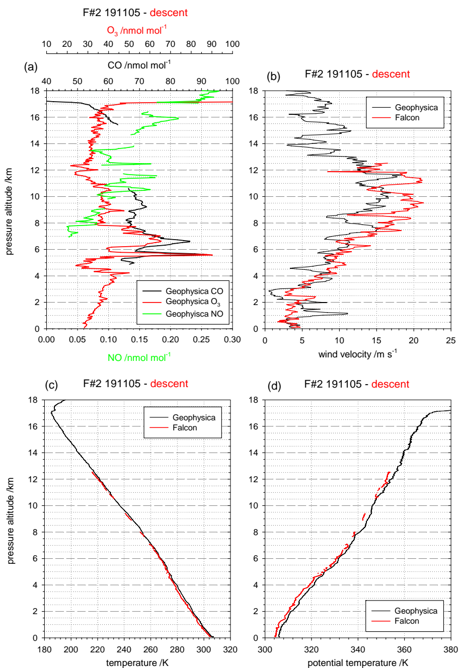
Fig. 12. Vertical profiles for CO, O 3 , and NO (a), wind velocity (b), temperature (c), and potential temperature (d) derived from measurements with the Falcon and Geophysica aircraft during descent on 19 November 2005.
