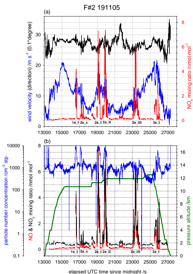
Fig. 5. Time series of NO x , wind velocity and direction in (a) and NO, NO y , CN, and pressure altitude in (b) for the Falcon flight on 19 November 2005. Anvil penetrations are labelled in black.
