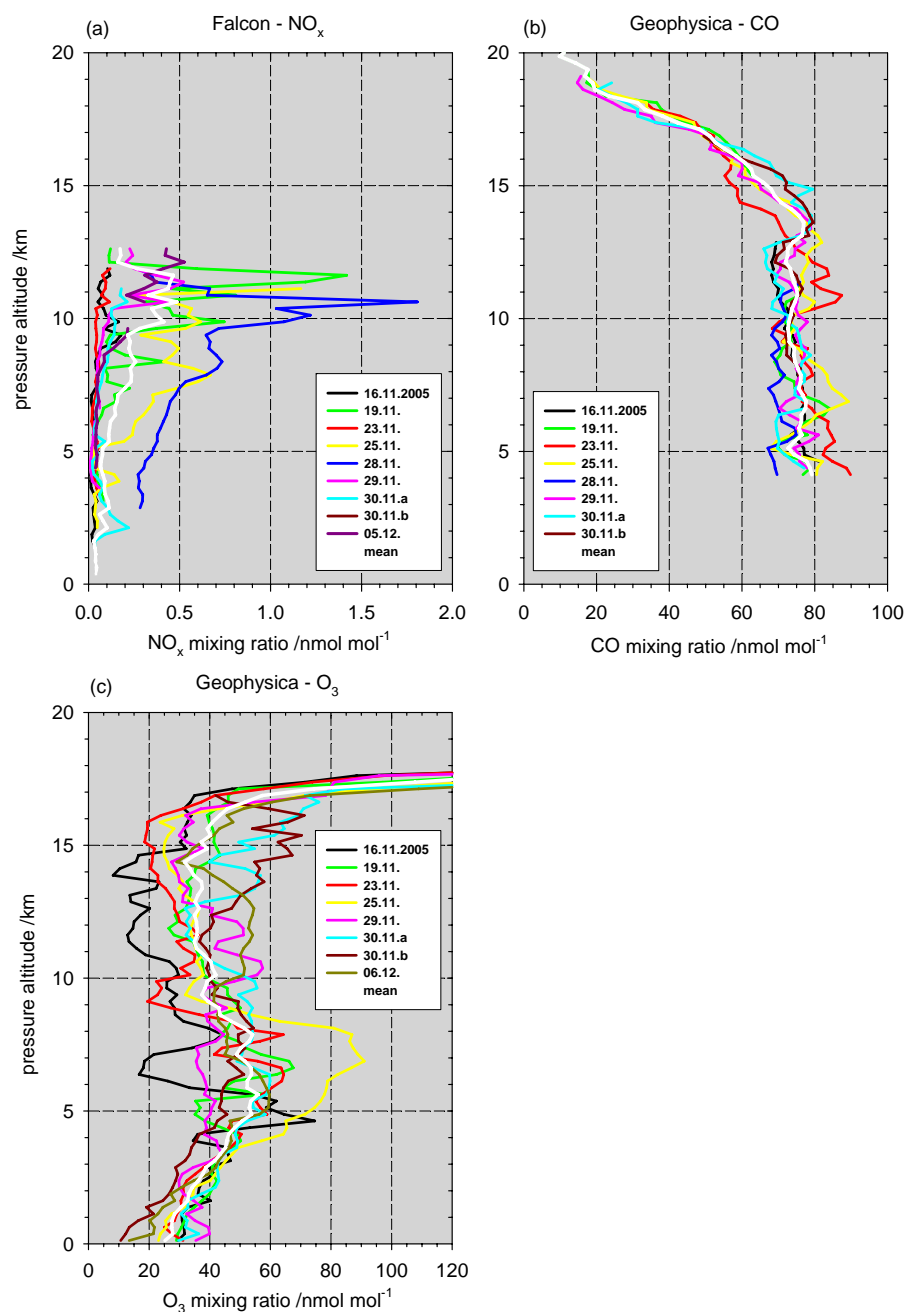
Fig. 9. Mean vertical profiles for NO x (a), CO (b), and O 3 (c) derived from measurements with the Falcon and Geophysica aircraft. Mean values for every 250 m altitude bin are given for all available SCOUT-O3 flights (dd:mm:(yyyy)) in colour. The white lines show the mean of all coloured flight profiles in each figure.
