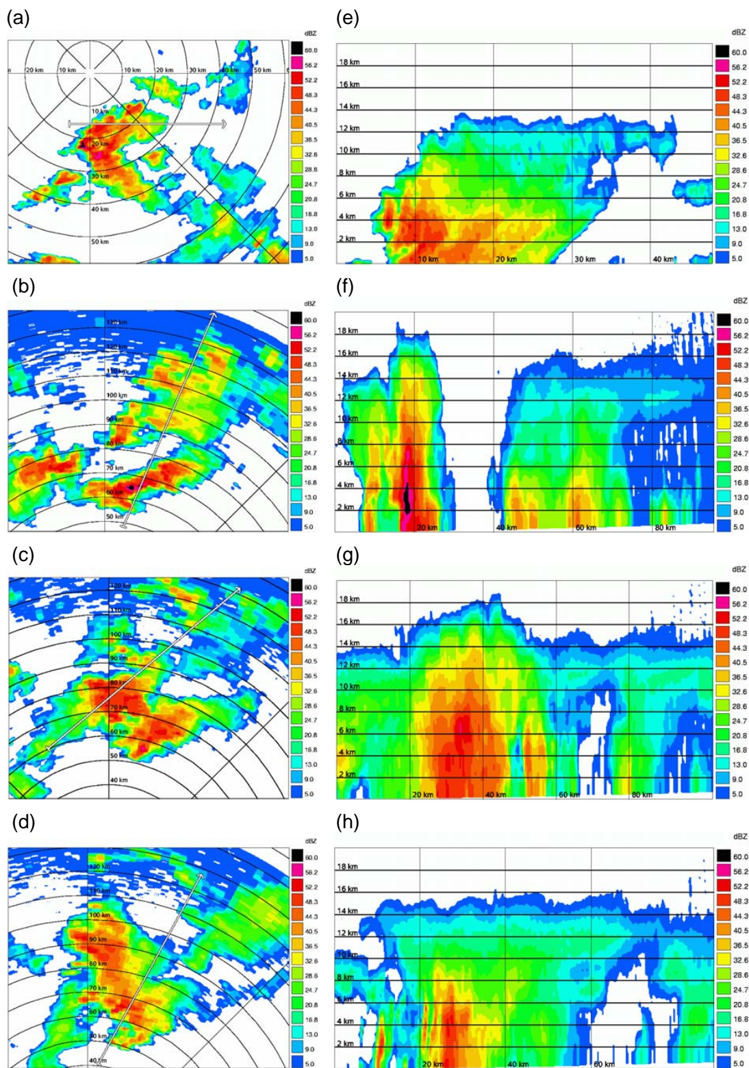
Fig. 13. Horizontal distribution of radar reflectivity (a–d) and the corresponding vertical cross-sections (e–h) along the white arrows indicated in (a–d) for the 19 November 2005 measured with the CPOL radar in Darwin. In (a) the focus is on thunderstorm “1a” at 04:30 UTC, in (b–d) the focus is on Hector pre-storm developments “2a_x” and the mature and dissipating Hector “2a_I-III” at 04:00 (b), 04:30 (c) and 05:00 (d) UTC.
