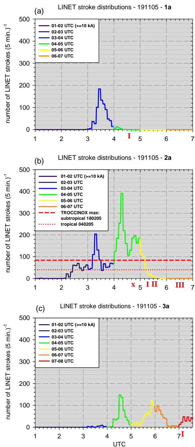
Fig. 8. Time series of LINET stroke rates (colour-coded as in Fig. 7) determined for the selected thunderstorm systems on 19 November 2005 labelled “1a” (a), “2a” (b), and “3a” (c) (only strokes with peak currents \geq 10 kA considered). The times when the different anvil penetrations took place are labelled in red below the time scale.
