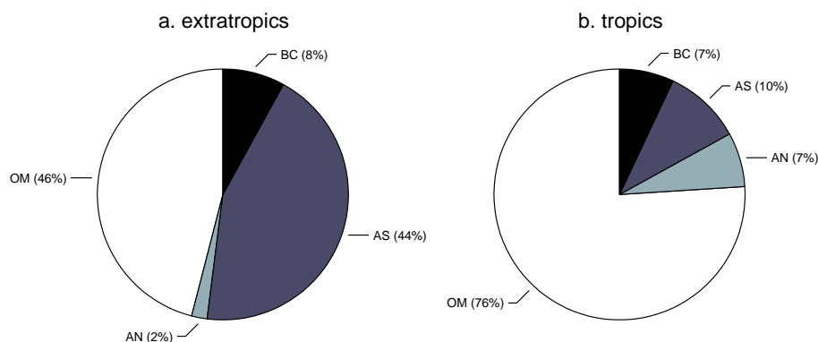
Fig. 2. Apportionment of PM 2.5 aerosol mass concentrations for (a) extratropical southern Africa and (b) tropical southern Africa. Shown are the median percent contributions of organic matter (OM), black carbon (BC), ammonium nitrate (AN), and ammonium sulfate (AS).
