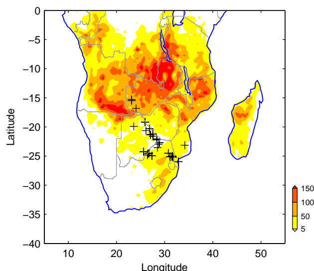
Fig. 1. Locations of filter samples collected during the SAFARI-2000 field campaign (black crosses) and used in this study. Colors are mean (2001–2007) August and September fire counts derived from Moderate Resolution Imaging Spectroradiometer (MODIS) measurements (Collection 5) in units of fires per half degree grid-cell.
