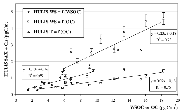
Fig. 6. Correlations between concentrations ( \mu\text{g C m}^{-3} ) of WSOC, OC, versus Water Soluble and Total and HULIS extracted with the C 18 +SAX protocol. Uncertainties include relative standard deviation of extraction efficiency determined with SRFA standard.
