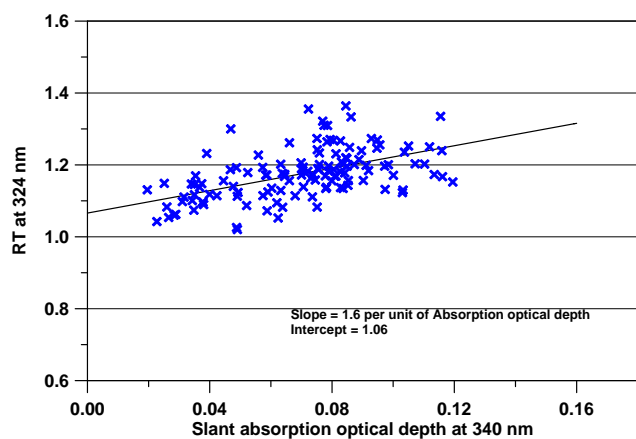
Fig. 4. OMI-GB ratio at 324 nm for cloudless cases as a function of AAOTS. The black line is a linear regression on the data.
