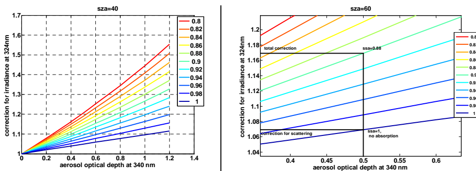
Fig. 5. Radiative model calculations of UV attenuation E_{\text{clear}(CT=1)}/E_{\text{aero}} , for various AOT and SSA values (left). The ratios E_{\text{clear}(CT=1)}/E_{\text{aero}} , for a constant solar zenith angle (60 degrees) and (\text{SSA}, \text{AOT}) = (0.88, 0.5) at 340 nm.
