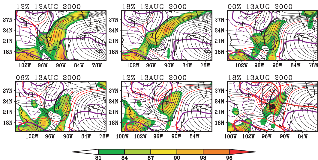
Fig. B9. Streamlines of horizontal flow at 850 hPa for the genesis sequence of Tropical Storm Beryl as in Fig. 28, with high values of ERA-40 saturation fraction indicated by shading (units: percent). The sequence of frames translates westward at the zonal propagation speed of the parent wave at 850 hPa ( -3.8 \pm 2.8 \text{ ms}^{-1} ) and streamlines are calculated and displayed in the co-moving frame.
