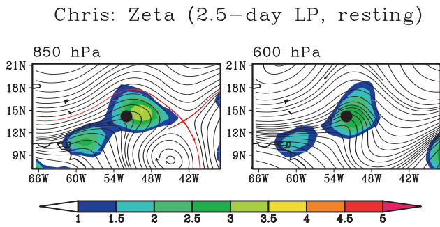
Fig. B3. Streamlines of horizontal flow at (a) 850 hPa and (b) 600 hPa at the genesis time of Tropical Storm Chris, in the resting frame. Shading indicates relative vorticity (units: 10^{-5} \text{ s}^{-1} ) which is invariant with respect to translation, therefore identical in co-moving and resting frames (cp. final panel of Figs. 23, 24).
