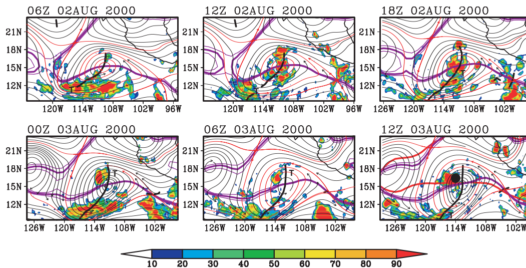
Fig. 13. Streamlines of horizontal flow at 600 hPa for the genesis sequence of Tropical Storm Fabio as in Fig. 11, with high values of TRMM 3-h accumulated precipitation indicated by shading (units: mm/day). The sequence of frames translates westward at the zonal propagation speed of the parent wave at 600 hPa ( -3.1 \pm 0.8 \text{ ms}^{-1} ) and streamlines are calculated and displayed in the co-moving frame.
