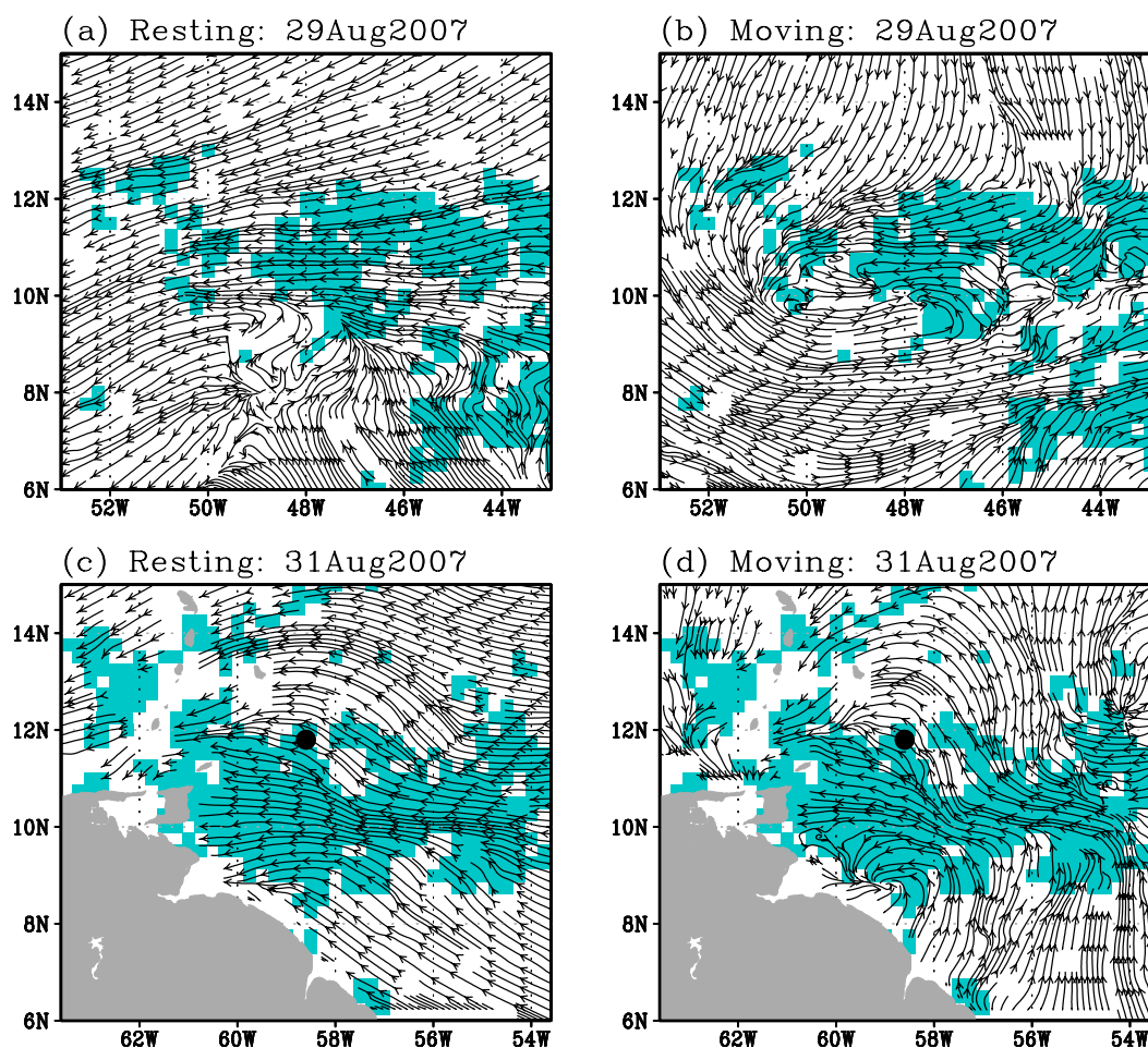
Fig. D1. Streamlines of surface flow obtained from QuikSCAT images of Hurricane Felix (2007) in late August 2007. (a, c) Resting frame; (b, d) co-moving frame ( C_p = -6.7 \pm 0.5 \text{ ms}^{-1} ). Regions of possible rain contamination are indicated by cyan shading.
