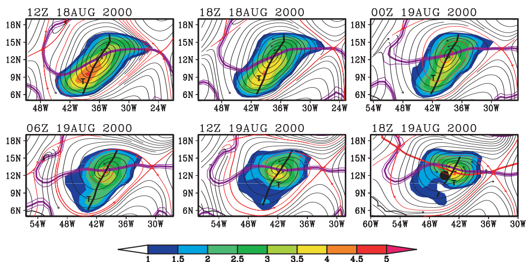
Fig. 6. Streamlines of horizontal flow for the genesis sequence of Hurricane Debby as in Fig. 5, but at 600 hPa. Shading indicates relative vorticity (units: 10^{-5} \text{ s}^{-1} ). The sequence of frames translates westward at the zonal propagation speed of the parent wave at 600 hPa ( -9.1 \pm 0.3 \text{ ms}^{-1} ) and streamlines are calculated and displayed in the co-moving frame.
