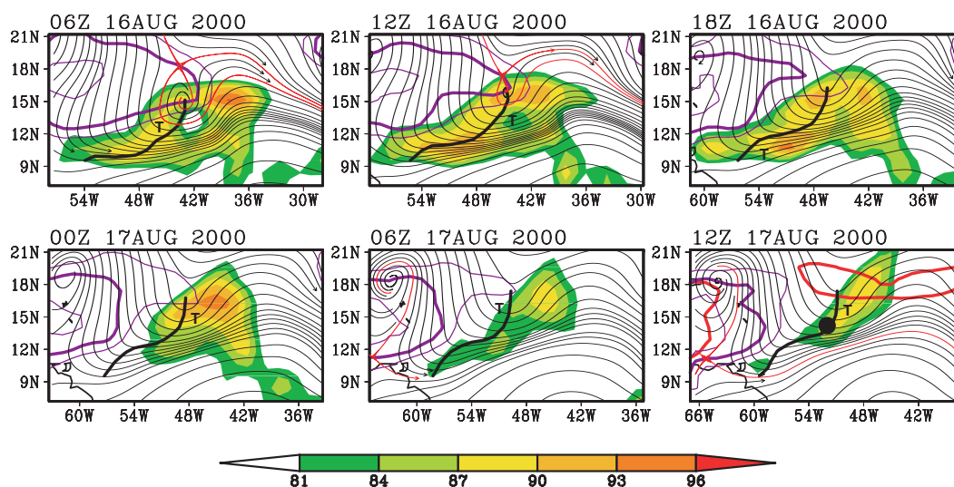
Fig. B4. Streamlines of horizontal flow at 850 hPa for the genesis sequence of Tropical Storm Chris as in Fig. 23, with high values of ERA-40 saturation fraction indicated by shading (units: percent). The sequence of frames translates westward at the zonal propagation speed of the parent wave at 850 hPa ( -9.1 \pm 1.1 \text{ m s}^{-1} ) and streamlines are calculated and displayed in the co-moving frame.
