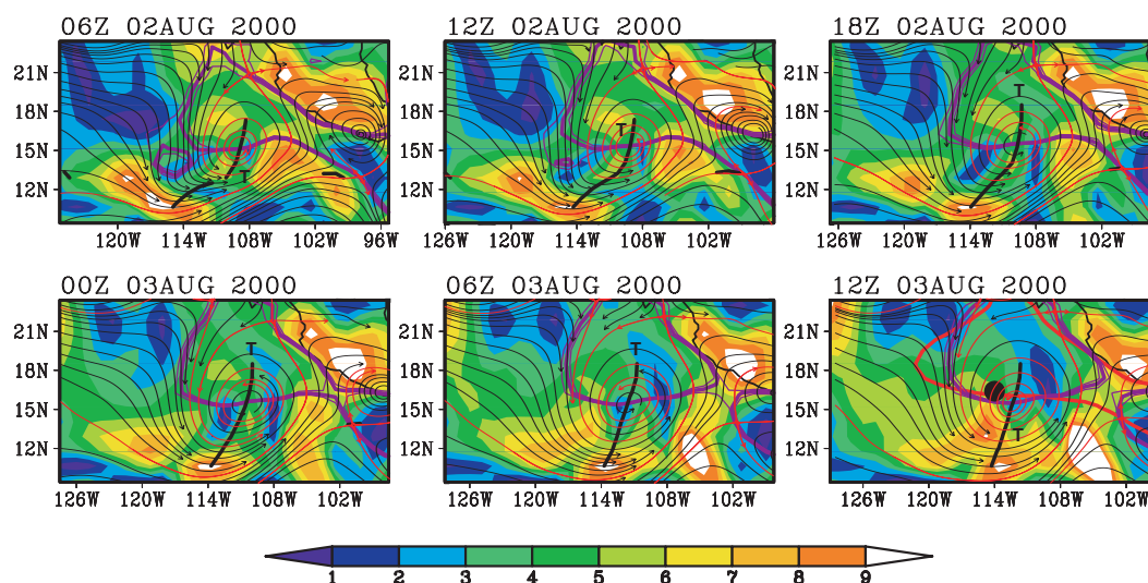
Fig. 14. Streamlines of horizontal flow at 850 hPa for the genesis sequence of Tropical Storm Fabio as in Fig. 10, with ERA-40 850–500 hPa vertical shear (magnitude of shear vector, units: \text{ms}^{-1} ) indicated by shading. The sequence of frames translates westward at the zonal propagation speed of the parent wave at 850 hPa ( -3.7 \pm 0.5 \text{ ms}^{-1} ) and streamlines are calculated and displayed in the co-moving frame.
