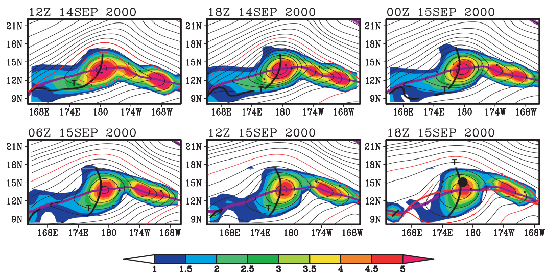
Fig. B11. Streamlines of horizontal (rotational + divergent) flow at 850 hPa, as seen in ERA-40 data, for six consecutive analyses leading up to the best-track genesis time of Super Typhoon Shanshan (2000). Shading indicates relative vorticity (units: 10^{-5} \text{ s}^{-1} ). The sequence of frames translates westward at the zonal propagation speed of the parent wave at 850 hPa as estimated from the Hovmöller method ( -2.8 \pm 0.3 \text{ ms}^{-1} ) and streamlines are calculated and displayed in the co-moving frame; note that relative vorticity itself is invariant with respect to the translation. Isopeleths of zero relative zonal flow are shown (purple) together with their uncertainty. In the final panel of the sequence the critical latitude of the parent wave is also indicated (red) corresponding to isopleths of zero relative zonal flow in low-frequency data with periods longer than 9 days. The wave's trough axis is shown for reference (black). The genesis location is indicated by the black dot in the final panel.
