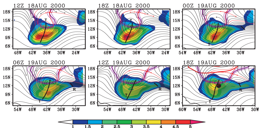
Fig. 5. Streamlines of horizontal (rotational + divergent) flow at 850 hPa, as seen in ERA-40 data, for six consecutive analyses leading up to the best-track genesis time of Hurricane Debby (2000). Shading indicates relative vorticity (units: 10^{-5} \text{ s}^{-1} ). The sequence of frames translates westward at the zonal propagation speed of the parent wave at 850 hPa as estimated from the Hovmöller method ( -10.0 \pm 0.6 \text{ ms}^{-1} ) and streamlines are calculated and displayed in the co-moving frame; note that relative vorticity itself is invariant with respect to the translation. Isopleths of zero relative zonal flow are shown (purple) together with their uncertainty. In the final panel of the sequence the critical latitude of the parent wave is also indicated (red) corresponding to isopleths of zero relative zonal flow in low-frequency data with periods longer than 9 days. The wave's trough axis is shown for reference (black). The genesis location is indicated by the black dot in the final panel.
