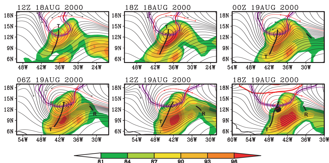
Fig. 8. Streamlines of horizontal flow at 850 hPa for the genesis sequence of Hurricane Debby as in Fig. 5, with high values of ERA-40 saturation fraction indicated by shading (units: percent). The sequence of frames translates westward at the zonal propagation speed of the parent wave at 850 hPa ( -10.0 \pm 0.6 \text{ ms}^{-1} ) and streamlines are calculated and displayed in the co-moving frame.
