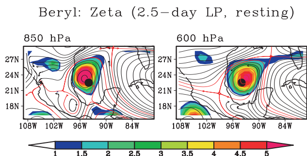
Fig. B8. Streamlines of horizontal flow at (a) 850 hPa and (b) 600 hPa at the genesis time of Tropical Storm Beryl, in the resting frame. Shading indicates relative vorticity (units: 10^{-5} \text{ s}^{-1} ) which is invariant with respect to translation, therefore identical in co-moving and resting frames (cp. final panels of Figs. 28, 29).
