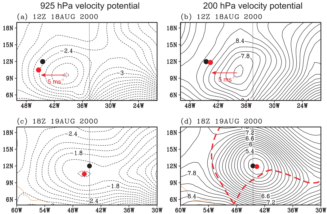
Fig. 21. Velocity potential of divergent flow, as seen in ERA-40 data, at (a, c) 925 hPa and (b, d) 200 hPa leading up to the genesis time of Hurricane Debby, at (a, b) 30 h before genesis and (c, d) genesis.
