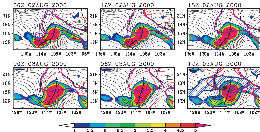
Fig. 10. Streamlines of horizontal (rotational + divergent) flow at 850 hPa, as seen in ERA-40 data, for six consecutive analyses leading up to the best-track genesis time of Tropical Storm Fabio (2000). Shading indicates relative vorticity (units: 10^{-5} \text{ s}^{-1} ). The sequence of frames translates westward at the zonal propagation speed of the parent wave at 850 hPa as estimated from the Hovmöller method ( -3.7 \pm 0.5 \text{ ms}^{-1} ) and streamlines are calculated and displayed in the co-moving frame; note that relative vorticity itself is invariant with respect to the translation. Isopleths of zero relative zonal flow are shown (purple) together with their uncertainty. In the final panel of the sequence the critical latitude of the parent wave is also indicated (red) corresponding to isopleths of zero relative zonal flow in low-frequency data with periods longer than 9 days. These data were also used to estimate the zero contour of absolute vorticity gradient or “effective \beta ” (blue). This quantity is negative in the zone just north of the genesis latitude, bracketed by the blue curves (diagonal hatching). The wave’s trough axis is shown for reference (black). The genesis location is indicated by the black dot in the final panel.
