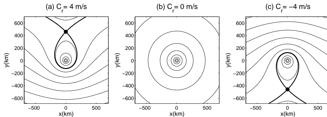
Fig. 3. Total streamline structure of a point vortex with cyclonic circulation \Gamma immersed in a constant mean zonal flow U_b . In the frame of reference displayed here (with zonal translation speed equal to zero) the vortex is spatially and temporally fixed at the origin. The total flow is given by the superposition of a constant background zonal wind and a circularly symmetric flow induced by the point vortex. This flow is an exact steady solution of the 2-D Euler equations. As noted in the text, identical streamline patterns are obtained in a resting basic state when the vortex translates zonally at speed C_p = -U_b . The numerical value of \Gamma is based on the gyre circulation analyzed for pre-Debby in August 2000. Three cases are sketched: (a) U_b = 4 \text{ ms}^{-1} (moderate westerly flow over the vortex), (b) U_b = 0 (zero background flow) and (c) U_b = -4 \text{ ms}^{-1} (moderate easterly flow). Light solid curves denote streamlines. The black dot denotes the stagnation point located at (X_c, Y_c) = (0, \Gamma/2\pi U_b) ; the fluid velocity vanishes there. The thick solid curve denotes the dividing streamline that divides the flow into three distinct regions: a core region near the vortex, upper outside region and lower outside region. As the magnitude of the imposed flow increases, the distance from the vortex center to the separatrix decreases and the amount of fluid isolated within the core region decreases.
