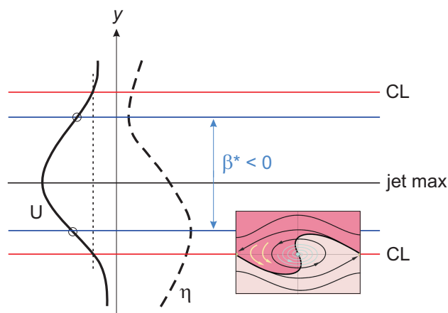
Fig. 2. Idealized profile of an easterly jet U north of the equator, on which stable easterly waves propagate westward having their critical latitudes just outside the jet's inflection points where the gradient of absolute vorticity \eta or “effective \beta ” is zero. Unstable waves may be imagined to have their critical latitudes just inside the latitude of inflection points.
