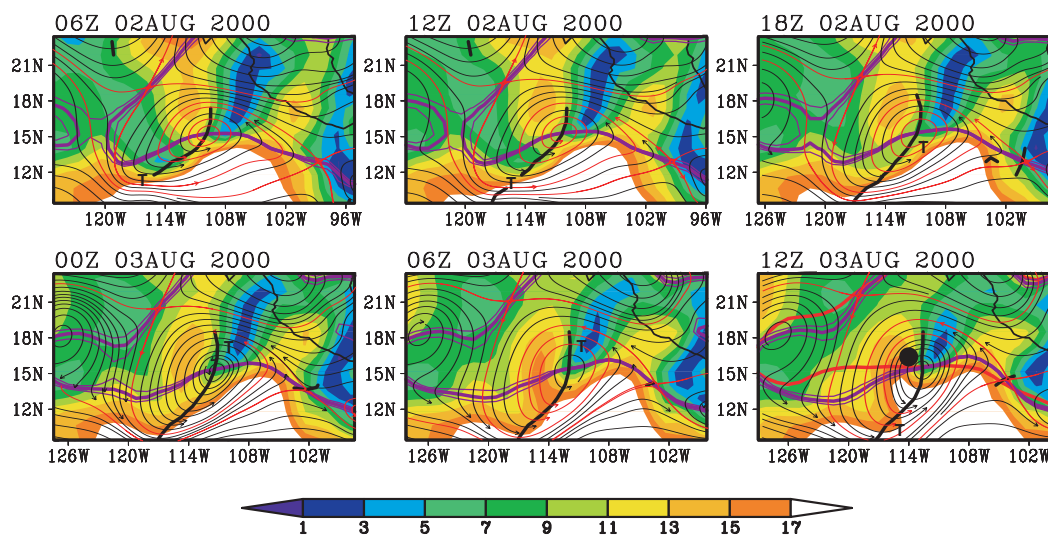
Fig. 15. Streamlines of horizontal flow at 600 hPa for the genesis sequence of Tropical Storm Fabio as in Fig. 11, with ERA-40 850–200 hPa vertical shear (magnitude of shear vector, units: \text{ms}^{-1} ) indicated by shading. The sequence of frames translates westward at the zonal propagation speed of the parent wave at 600 hPa ( -3.1 \pm 0.8 \text{ ms}^{-1} ) and streamlines are calculated and displayed in the co-moving frame.
