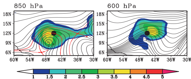
Fig. 7. Streamlines of horizontal flow at (a) 850 hPa and (b) 600 hPa at the genesis time of Hurricane Debby, in the resting frame. Shading indicates relative vorticity (units: 10^{-5} \text{ s}^{-1} ) which is invariant with respect to translation, therefore identical in co-moving and resting frames (cp. final panels of Figs. 5, 6).
