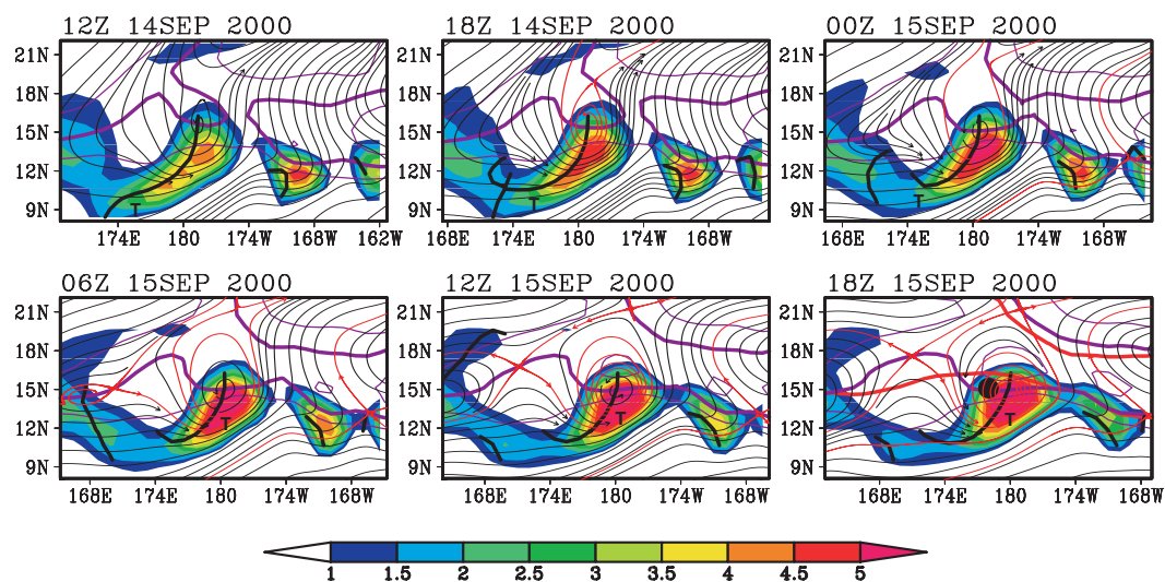
Fig. B12. Streamlines of horizontal flow for the genesis sequence of Super Typhoon Shanshan as in Fig. 33, but at 600 hPa. Shading indicates relative vorticity (units: 10^{-5} \text{ s}^{-1} ). The sequence of frames translates westward at the zonal propagation speed of the parent wave at 600 hPa ( -5.7 \pm 2.8 \text{ ms}^{-1} ) and streamlines are calculated and displayed in the co-moving frame.
