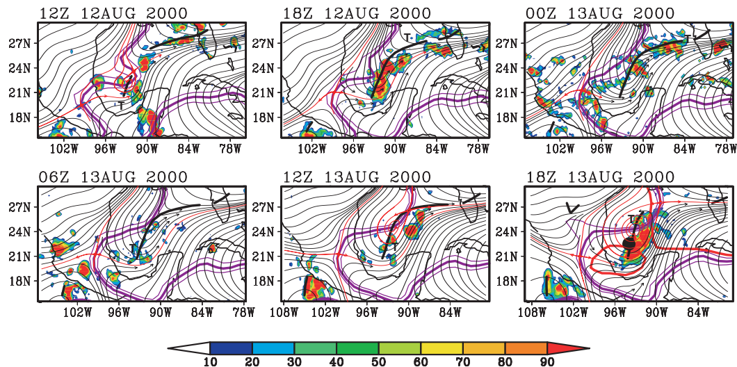
Fig. B10. Streamlines of horizontal flow at 600 hPa for the genesis sequence of Tropical Storm Beryl as in Fig. 29, with high values of TRMM 3-h accumulated precipitation indicated by shading (units: mm/day). The sequence of frames translates westward at the zonal propagation speed of the parent wave at 600 hPa ( -3.1 \pm 0.8 \text{ ms}^{-1} ) and streamlines are calculated and displayed in the co-moving frame.
