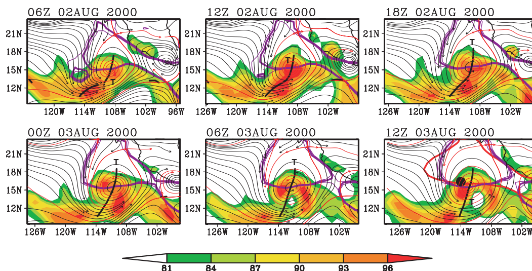
Fig. 12. Streamlines of horizontal flow at 850 hPa for the genesis sequence of Tropical Storm Fabio as in Fig. 10, with high values of ERA-40 saturation fraction indicated by shading (units: percent). The sequence of frames translates westward at the zonal propagation speed of the parent wave at 850 hPa ( -3.7 \pm 0.5 \text{ ms}^{-1} ) and streamlines are calculated and displayed in the co-moving frame.
