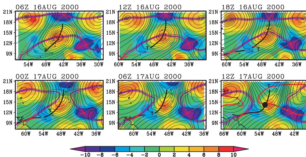
Fig. B2. Stream function of horizontal flow for the genesis sequence of Tropical Storm Chris as in Fig. 23, but at 600 hPa. Shading indicates the Okubo-Weiss parameter (units: 10^{-10} \text{ s}^{-2} ) as defined in Eq. (2). This quantity, like vorticity, is invariant with respect to translation, therefore identical in co-moving and resting frames. The sequence of frames translates westward at the zonal propagation speed of the parent wave at 600 hPa ( -8.5 \pm 0.5 \text{ ms}^{-1} ) and stream function is calculated and displayed in the co-moving frame.
