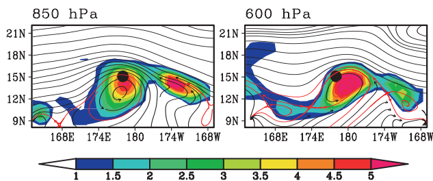
Fig. B13. Streamlines of horizontal flow at (a) 850 hPa and (b) 600 hPa at the genesis time of Super Typhoon Shanshan, in the resting frame. Shading indicates relative vorticity (units: 10^{-5} \text{ s}^{-1} ) which is invariant with respect to translation, therefore identical in co-moving and resting frames (cp. final panels of Figs. 33, 34).
