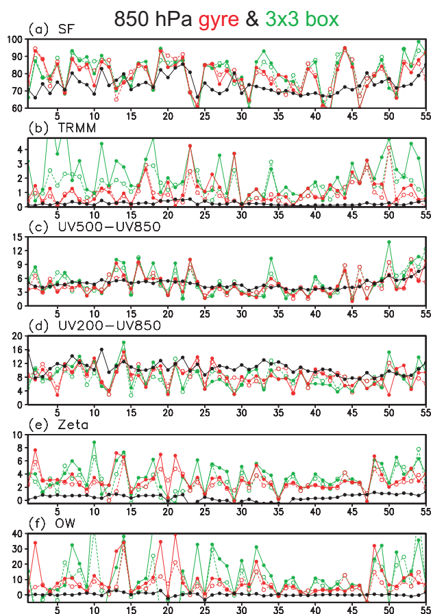
Fig. 16. Spatio-temporal average of dynamical and thermodynamical fields in the neighborhood of the best-track genesis location and time immediately preceding. The storms are arrayed west to east, from left to right, in the reverse of Table 1. The spatial average corresponds either to that of (i) the translating gyre (red) or (ii) a 3 \times 3 matrix of ERA-40 grid points surrounding the point x(t) = x_0 - C_p \cdot (t - t_0) where x is longitude, t is time, C_p is the speed of translation and the subscript 0 refers to the location and time of genesis (green). The temporal average corresponds either to (i) the genesis time (single analysis, filled circles) or (ii) the 36-h interval preceding and slightly overlapping genesis time (average of six consecutive 6-hourly analyses ending at genesis time, open circles). Black circles denote “climatological” values for August–September 1998–2001 at the various gyre or grid box locations. The data shown in the figure were derived using gyre properties and translation speeds at 850 hPa: (a) saturation fraction averaged from 1000–500 hPa (units: percent), (b) TRMM deep convective precipitation (units: mm/day), (c) vertical shear from lower to mid-troposphere (850 to 500 hPa, units: \text{ms}^{-1} ), (d) vertical shear from lower to upper troposphere (850 to 200 hPa, units: \text{ms}^{-1} ), (e) relative vorticity at 850 hPa (units: 10^{-5} \text{ s}^{-1} ), (f) Okubo-Weiss parameter at 850 hPa (units: 10^{-10} \text{ s}^{-2} ). Please refer to footnote 25 for important information regarding the climatology of vertical shear and Okubo-Weiss.
