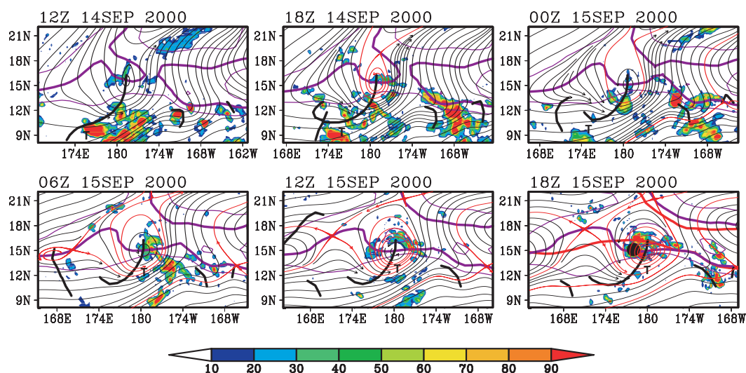
Fig. B14. Streamlines of horizontal flow at 600 hPa for the genesis sequence of Super Typhoon Shanshan as in Fig. 34, with high values of TRMM 3-h accumulated precipitation indicated by shading. Units: mm/day. The sequence of frames translates westward at the zonal propagation speed of the parent wave at 600 hPa ( -5.7 \pm 2.8 \text{ ms}^{-1} ) and streamlines are calculated and displayed in the co-moving frame.
