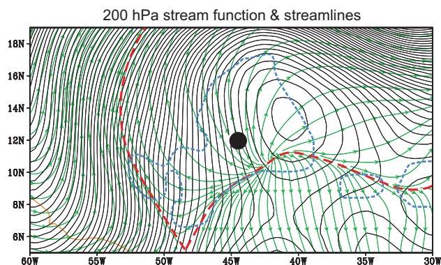
Fig. 19. Streamlines of horizontal flow and stream function of non-divergent flow at 200 hPa calculated and displayed in a frame of reference moving 5 \text{ms}^{-1} westward, at the genesis time of Hurricane Debby. Divergence contributing to anticyclonic outflow can be seen by comparing streamlines with stream function. The genesis location is indicated by the black dot; TRMM precipitation is outlined in blue.
