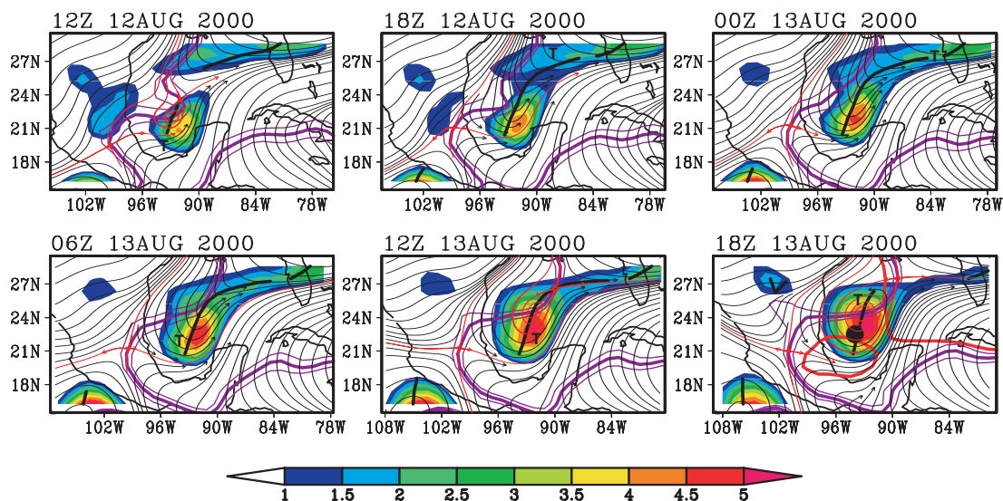
Fig. B7. Streamlines of horizontal flow for the genesis sequence of Tropical Storm Beryl as in Fig. 28, but at 600 hPa. Shading indicates relative vorticity (units: 10^{-5} \text{ s}^{-1} ). The sequence of frames translates westward at the zonal propagation speed of the parent wave at 600 hPa ( -3.1 \pm 0.8 \text{ ms}^{-1} ) and streamlines are calculated and displayed in the co-moving frame.
