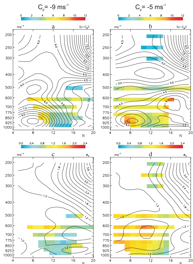
Fig. 20. Horizontal wind speed in two co-moving frames averaged over the six consecutive analyses leading up to the genesis time of Hurricane Debby. The range of longitudes x used to construct the average is given by the speed of translation beginning at the genesis longitude ( x_0 = 44.5^\circ W) and going eastward (backward) in longitude (time) from the genesis point according to the formula x(t) = x_0 - C_p \cdot (t - t_0) where t_0 is the best-track genesis time. The horizontal wind speed in each co-moving frame is given by |\mathbf{U} - C_p \hat{\mathbf{i}}| where \mathbf{U} is the horizontal vector wind, C_p is translation speed and \hat{\mathbf{i}} is the unit vector in the x -direction. The quantity contoured represents a zonal average within \pm 15^\circ longitude of the center longitude as given above, including regions inside and outside the gyre. (a, c) C_p = -9 \text{ ms}^{-1} ; (b, d) C_p = -5 \text{ ms}^{-1} (negative values are westward). These values correspond approximately to the zonal component of disturbance propagation in the lower and upper troposphere, respectively. The maximum extent of closed stream function gyre in each frame of reference is also shown by superposing (as shaded pixels) the gyre-average values of |\mathbf{U} - C_p \hat{\mathbf{i}}| where they exist. Here, “gyre average” refers to a zonal average over longitudes within a closed gyre as delimited by a bounding contour of stream function \psi intersecting the nearest (in \psi ) separatrix. The lower panels show the temporal standard deviation of horizontal wind speed in each co-moving frame. The quantity contoured once again represents a zonal average over the entire domain, while shaded pixels indicate gyre-average values. For modulus and standard deviation, their zonal average was obtained by first summing the squares and then taking the square root of the sum.
