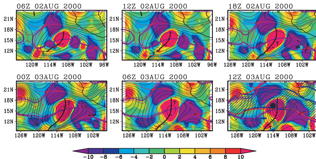
Fig. 11. Stream function of horizontal flow for the genesis sequence of Tropical Storm Fabio as in Fig. 10, but at 600 hPa. Shading indicates the Okubo-Weiss parameter (units: 10^{-10} \text{ s}^{-2} ) as defined in Eq. (2). This quantity, like vorticity, is invariant with respect to translation, therefore identical in co-moving and resting frames. The sequence of frames translates westward at the zonal propagation speed of the parent wave at 600 hPa ( -3.1 \pm 0.8 \text{ ms}^{-1} ) and stream function is calculated and displayed in the co-moving frame. Red and blue lines in the final panel show the wave’s critical latitude and isopleth of zero effective \beta as estimated from low-frequency data with periods longer than 9 days.
