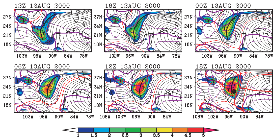
Fig. B6. Streamlines of horizontal (rotational + divergent) flow at 850 hPa, as seen in ERA-40 data, for six consecutive analyses leading up to the best-track genesis time of Tropical Storm Beryl (2000). Shading indicates relative vorticity (units: 10^{-5} \text{ s}^{-1} ). The sequence of frames translates westward at the zonal propagation speed of the parent wave at 850 hPa as estimated from the Hovmöller method ( -3.8 \pm 2.8 \text{ ms}^{-1} ) and streamlines are calculated and displayed in the co-moving frame; note that relative vorticity is invariant with respect to the translation. Isopleths of zero relative zonal flow are shown (purple) together with their uncertainty. In the final panel of the sequence the critical latitude of the parent wave is also indicated (red) corresponding to isopleths of zero relative zonal flow in low-frequency data with periods longer than 9 days. The wave's trough axis is shown for reference (black). The genesis location is indicated by the black dot in the final panel.
