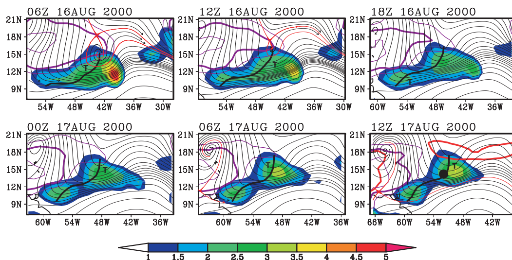
Fig. B1. Streamlines of horizontal (rotational + divergent) flow at 850 hPa, as seen in ERA-40 data, for six consecutive analyses leading up to the best-track genesis time of Tropical Storm Chris (2000). Shading indicates relative vorticity (units: 10^{-5} \text{ s}^{-1} ). The sequence of frames translates westward at the zonal propagation speed of the parent wave at 850 hPa as estimated from the Hovmöller method ( -9.1 \pm 1.1 \text{ ms}^{-1} ) and streamlines are calculated and displayed in the co-moving frame; note that relative vorticity itself is invariant with respect to the translation. Isopleths of zero relative zonal flow are shown (purple) together with their uncertainty. In the final panel of the sequence the critical latitude of the parent wave is also indicated (red) corresponding to isopleths of zero relative zonal flow in low-frequency data with periods longer than 9 days. The wave's trough axis is shown for reference (black). The genesis location is indicated by the black dot in the final panel.
