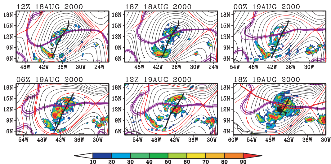
Fig. 9. Streamlines of horizontal flow at 600 hPa for the genesis sequence of Hurricane Debby as in Fig. 6, with high values of TRMM 3-h accumulated precipitation indicated by shading (units: mm/day). The sequence of frames translates westward at the zonal propagation speed of the parent wave at 600 hPa ( -9.1 \pm 0.3 \text{ ms}^{-1} ) and streamlines are calculated and displayed in the co-moving frame.
