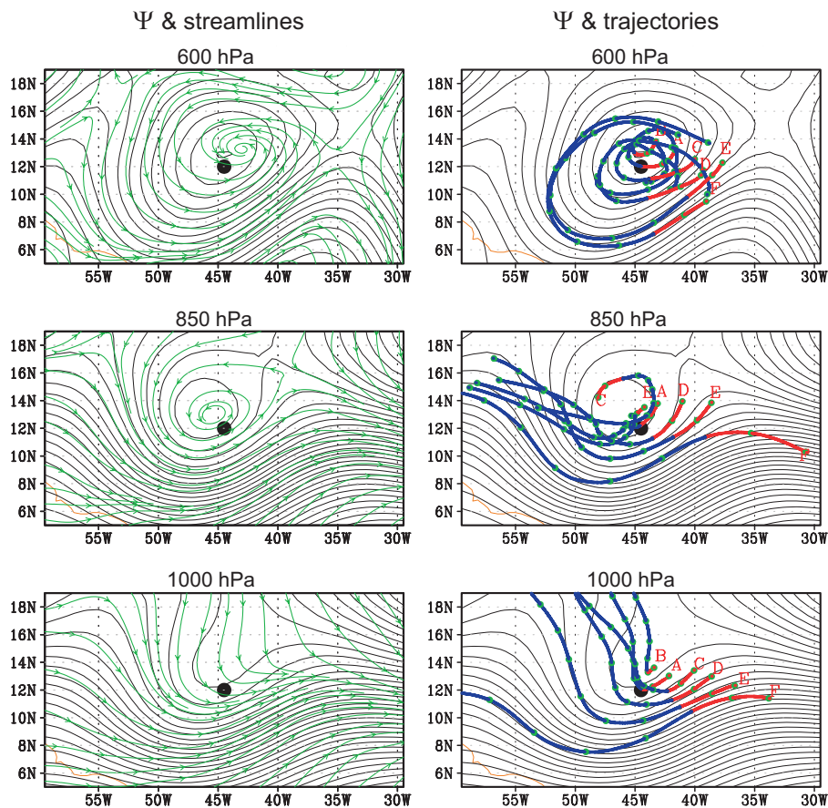
Fig. 18. Streamlines and trajectories of horizontal (rotational + divergent) flow at (a, b) 600 hPa, (c, d) 850 hPa, and (e, f) 1000 hPa as seen in ERA-40 data, for the average of six consecutive leading up to the best-track genesis time of Hurricane Debby (2000). As in Fig. 5, the streamlines (shown in panels a, c, e) are calculated and displayed in a frame of reference moving westward with the parent wave. Translation speeds estimated from the Hovmöller method at the three levels are -9.1 \pm 0.3 \text{ ms}^{-1} (600 hPa), -10.0 \pm 0.6 \text{ ms}^{-1} (850 hPa) and -10.1 \pm 0.6 \text{ ms}^{-1} (1000 hPa). Likewise the stream function of non-divergent flow (thin solid) and trajectories (shown in panels b, d, f) are calculated and is displayed in the co-moving frame. The contour interval for stream function is 0.5 \times 10^6 \text{ m}^2 \text{ s}^{-1} . The genesis location is indicated by the black dot in each panel. Note that owing to the translation of sequential frames used to construct the time average when C_p \neq 0 , the longitude labels on the x-axis pertain to the final analysis time only.
