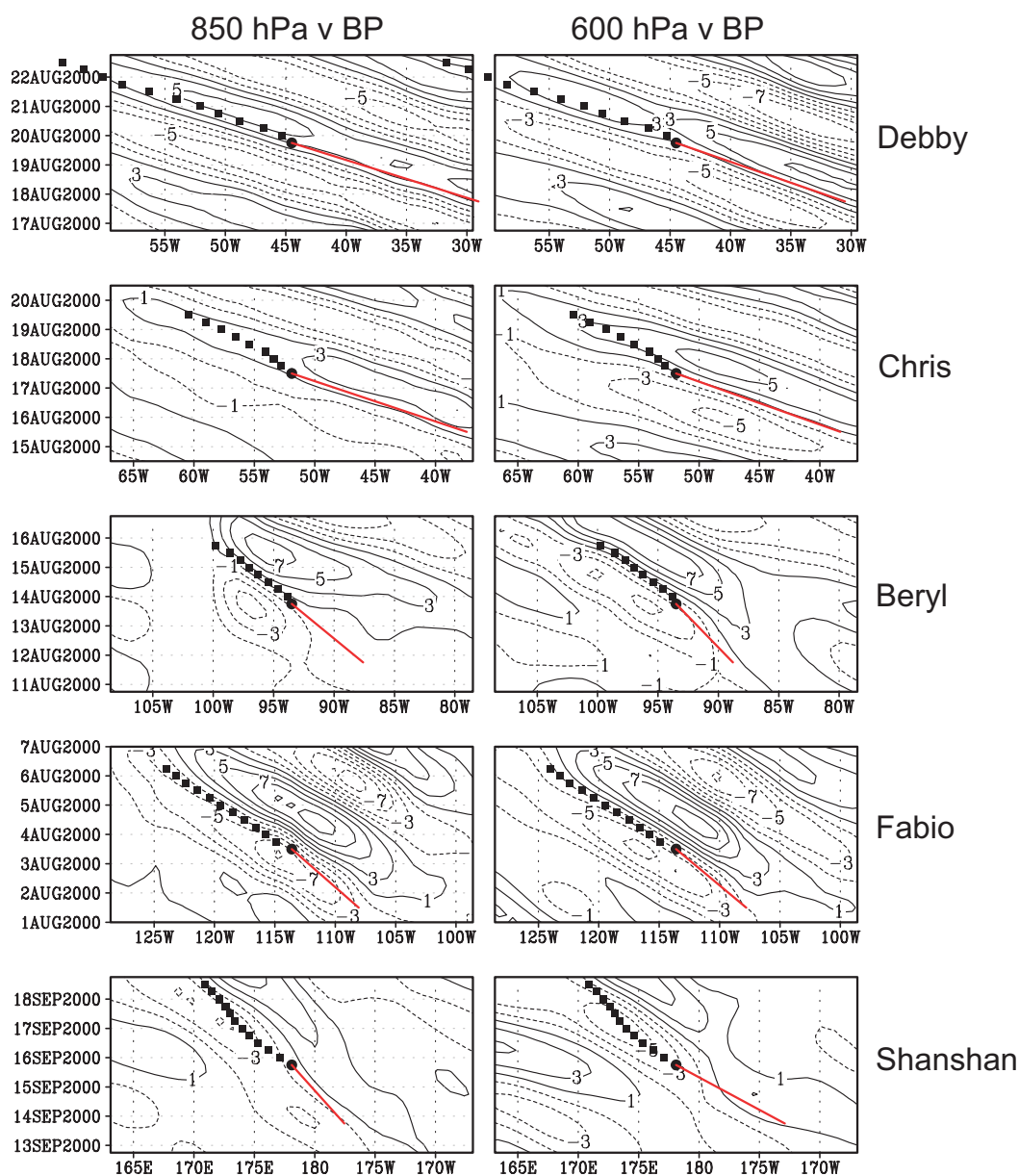
Fig. 4. Hovmöller plots of band-pass meridional velocity component at 850 hPa (left column) and 600 hPa (right column) in a longitude-time plane for the five cases of summer 2000 highlighted in the text: (a) Hurricane Debby; (b) Tropical Storm Chris; (c) Tropical Storm Beryl; (d) Tropical Storm Fabio; (e) Super Typhoon Shanshan. Black circles indicate the best-track longitude and time of genesis, while black squares indicate subsequent best track locations at 6-h intervals. Red line denotes the Hovmöller estimate of zonal translation speed C_p .
