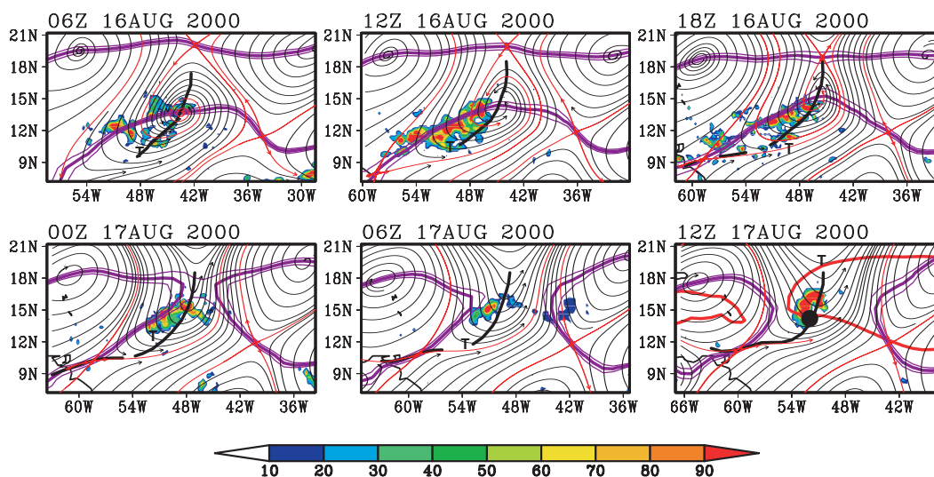
Fig. B5. Streamlines of horizontal flow at 600 hPa for the genesis sequence of Tropical Storm Chris as in Fig. 24, with high values of TRMM 3-h accumulated precipitation indicated by shading (units: mm/day). The sequence of frames translates westward at the zonal propagation speed of the parent wave at 600 hPa ( -8.5 \pm 0.5 \text{ m s}^{-1} ) and streamlines are calculated and displayed in the co-moving frame.
