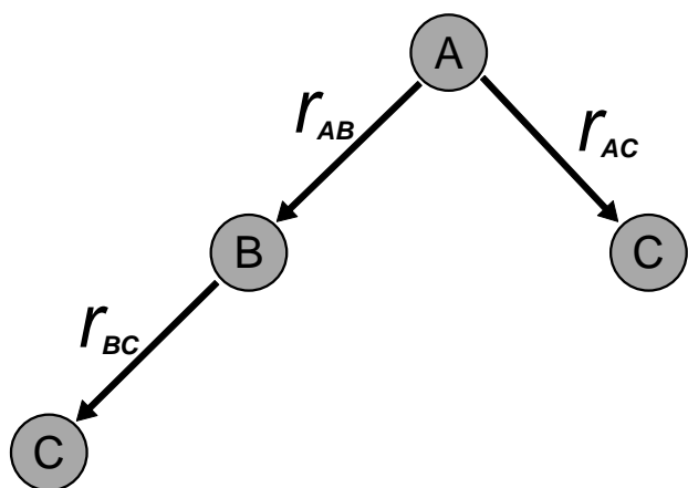
Fig. 1. Interaction graph for three species, in which Species A depends on C both directly and indirectly. Modified from Pepiot-Desjardins and Pitsch (2008).
