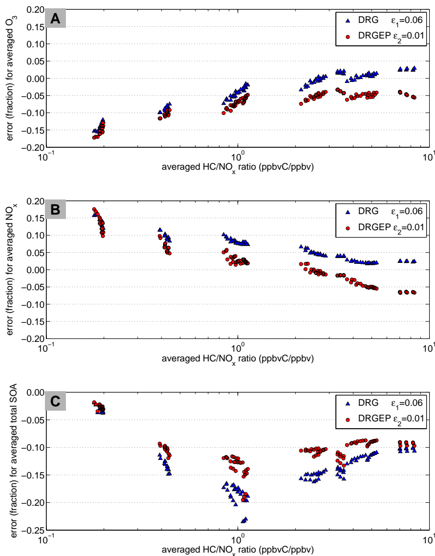
Fig. 3. Evaluation of averaged O 3 (panel A), averaged NO x (panel B), and averaged total SOA (panel C) from the two reduced mechanisms, against the reference mechanism by using DRG and DRGEP methods, respectively.
