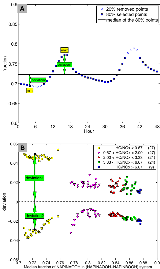
Fig. 2. One species (NAPINAOOH) in a two species system (NAPINAOOH+NAPINBOOH) in the gas phase: (A) fraction from one selected scenario, in which median value and errors for this scenario are calculated; (B) median fraction from 108 selected scenarios covering different HC/NO x (ppbv/ppbv) regimes.
