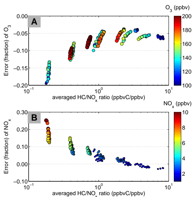
Fig. 7. Errors of the O_3 and NO_x between the final reduced lumping mechanisms and the reference mechanism from the 243 scenarios.
