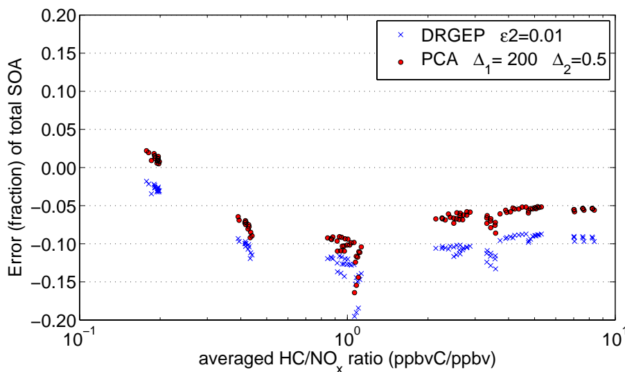
Fig. 4. Evaluations of the DRGEP and PCA methods for the average total SOA mass. In PCA, the thresholds are 200.0 for eigenvalue ( \Delta_1 ) and 0.5 for eigenvector ( \Delta_2 ).
