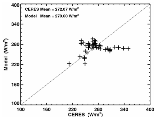
Fig. 6. Comparison of the modeled simultaneous TOA shortwave flux with CERES observations along the CALIPSO orbit over the Taklimakan Desert region ( 35^{\circ}\text{N} – 45^{\circ}\text{N} ) on 24, 26, 29, and 31 July 2006.
