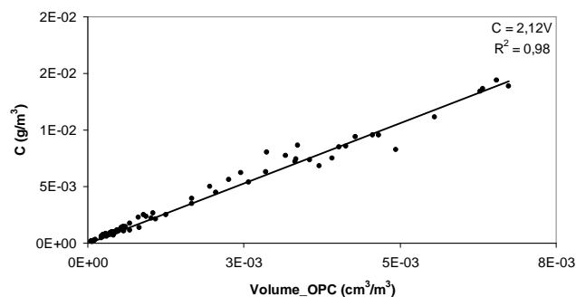
Fig. 3. Illustration of the good consistency ( r^2=0.98 ) between the mass concentration (C) recorded directly with a TEOM microbalance and the volume concentration reconstructed from the size-resolved number concentration measurements made with an optical particle counter. The data used in this figure are those acquired at the lowest measurements level during ME1. The slope of the straight line (2.12) is the particle's equivalent mass density.
