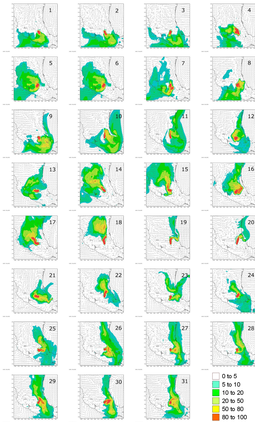
Fig. 2. Calculated effect of Mexico City emissions on 18Z mixing ratios of \text{NO}_y for 1–31 March 2006, shown as the % contribution for the near surface layer. Contribution calculated as percent difference between simulated values with and without Mexico City emissions.
