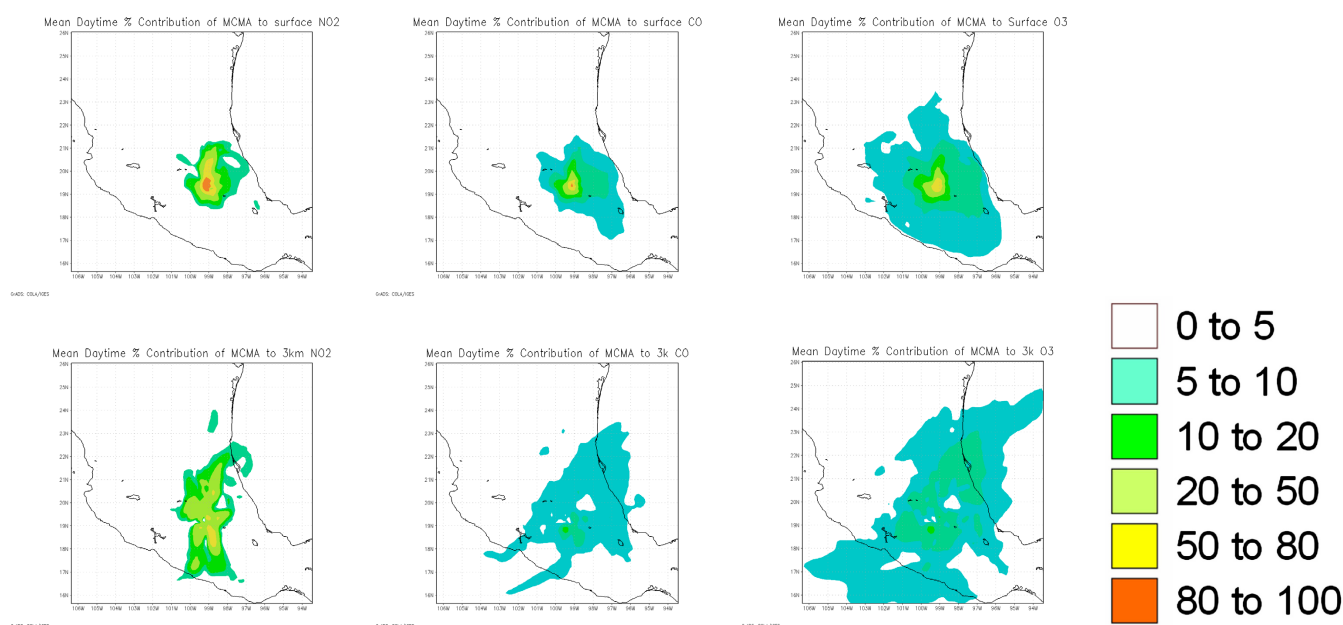
Fig. 1. Calculated effect of Mexico City on mean 18Z mixing ratios for March 2006. Top left: Mean % contribution to near surface NO 2 . Top center: CO. Top right: O 3 . Bottom left: Mean % contribution to NO 2 for 3 km above surface level. Top center: CO. Top right: O 3 . Contribution calculated as difference between simulated values with and without Mexico City emissions.
