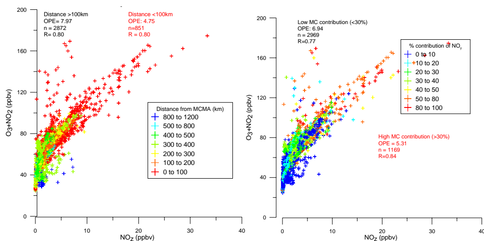
Fig. 6. Observed ozone production efficiencies, derived from O_3+NO_2 and NO_z observations as a function of distance (Left) and modeled influence of Mexico City emissions (Right) for all C-130 flights.
