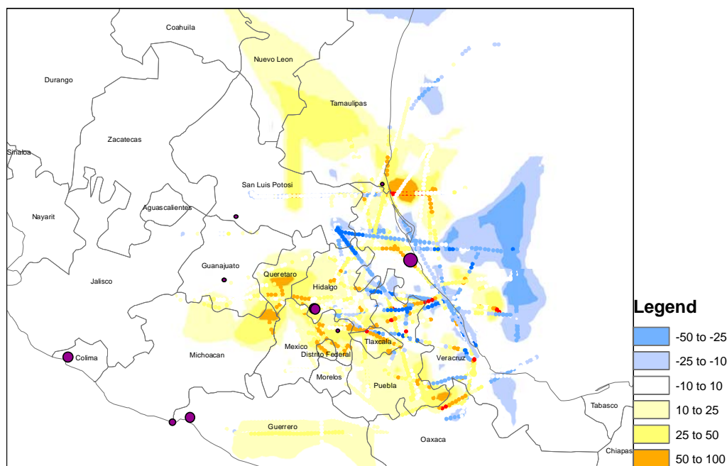
Fig. 8. Interpolated point percent bias of J[\text{NO}_2 \rightarrow \text{NO} + \text{O}] modeling for values extracted along C-130 flight tracks using kriging, n=3500 for all science flights.
