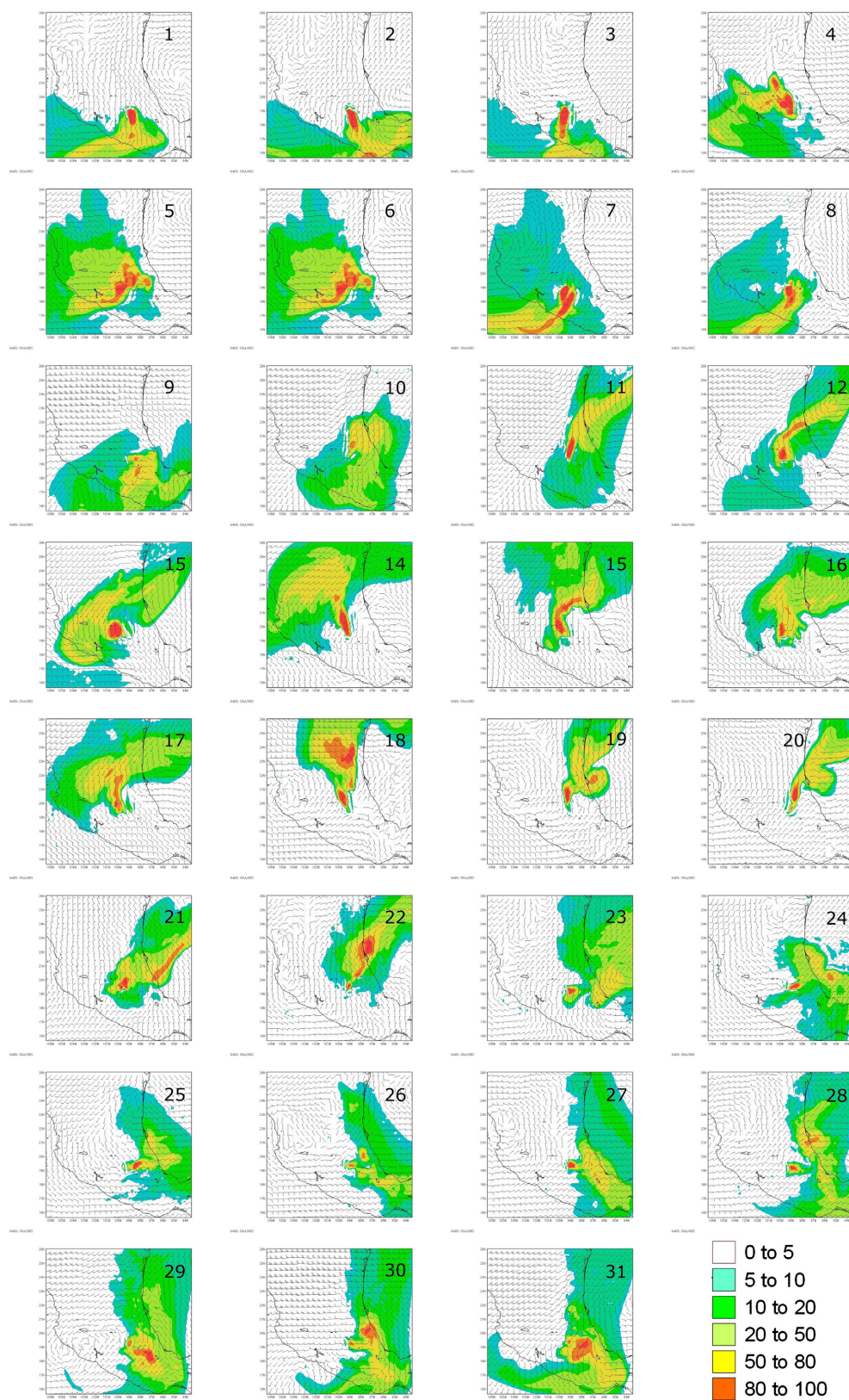
Fig. 3. Calculated effect of Mexico City emissions on 18Z mixing ratios of \text{NO}_y for 1–31 March 2006, shown as the % contribution for the 3 km above surface vertical layer. Contribution calculated as percent difference between simulated values with and without Mexico City emissions.
