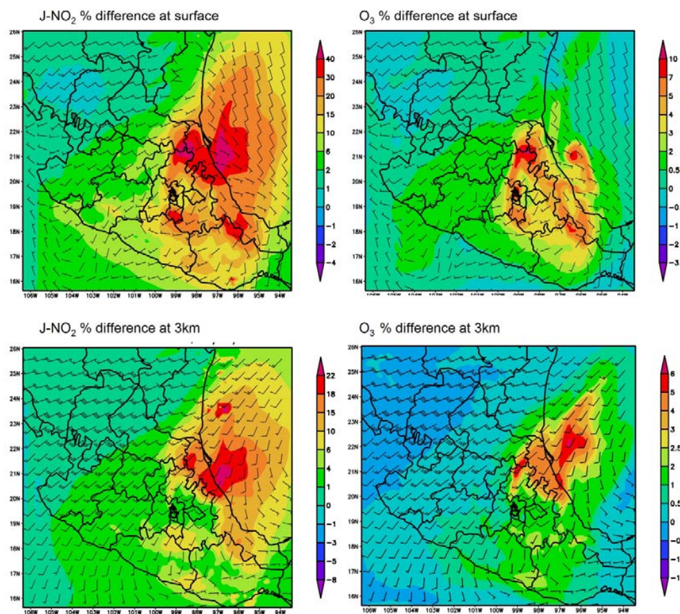
Fig. 7. Calculated modeled effect of aerosol loading on photolysis rate of \text{NO}_2 and \text{O}_3 formation calculated as difference between model runs with and without aerosol (NOAOD vs. base case) for 12 km STEM, 10 March 2006, at 21:00 UTC. Top panels calculated at surface layer; Bottom panels calculated at 3 km.
