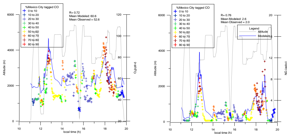
Fig. 5. Time series of observed and predicted O_3 and NO_y along 19 March 2006 C-130 flight track. Points are colored by the contribution of Mexico City tracer CO to total tracer CO. Left: O_3 (ppbv), Right: NO_y (ppbv).
