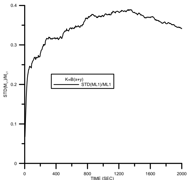
Fig. 11. The ratio of the standard deviation to expectation value of the largest droplet STD(M_{L1})/M_{L1} as a function of time for the approximating polynomial K(x, y) = B(x + y) , ( B = 8.82 \times 10^2 \text{ cm}^3 \text{ g}^{-1} \text{ s}^{-1} ).
