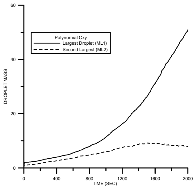
Fig. 2. Average time evolution for 1000 simulations versus time ( N_0=100 ) of the largest and second largest droplets for the kernel Cxy ( C=5.49 \times 10^{10} \text{ cm}^3 \text{ g}^{-2} \text{ s}^{-1} ).
