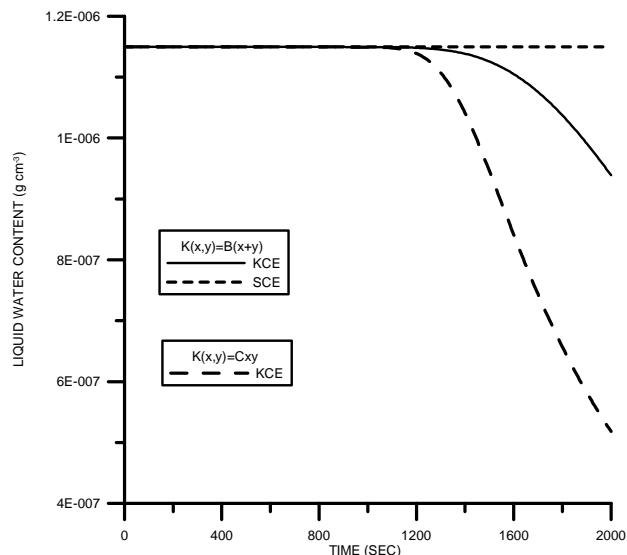
Fig. 12. Time evolution of the liquid water content (first moment of the distribution) for the sum kernel ( K(x, y) = B(x + y) ), calculated from size distributions of the KCE and true averages from the SCE, and for product kernel ( K(x, y) = Cxy ), calculated from the analytical solution of the KCE.
