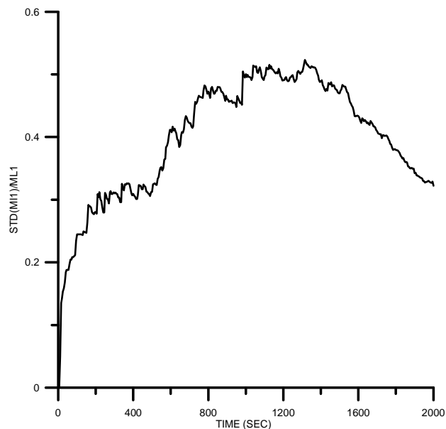
Fig. 3. The ratio of the standard deviation to expectation value of the largest droplet \text{STD}(M_{L1})/M_{L1} as a function of time.
