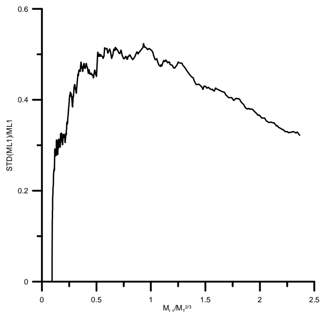
Fig. 4. The ratio of the standard deviation to expectation value of the largest droplet \text{STD}(M_{L1})/M_{L1} as a function of M_{L1}/M_T^{2/3} .
