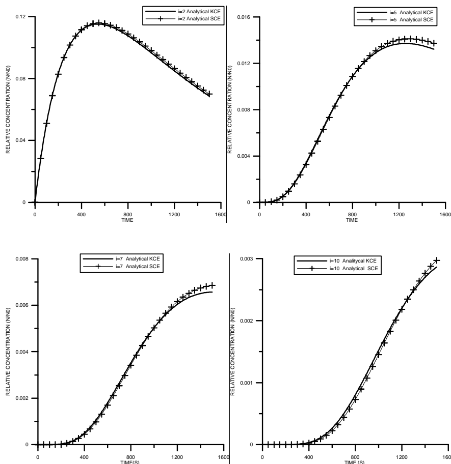
Fig. 10. Time evolution (bin sizes 2,5,7 and 10) for a system modeled by the sum kernel, as a function of time. The solid lines are the analytical solution of the KCE, the symbols are the analytical solutions of the SCE.
