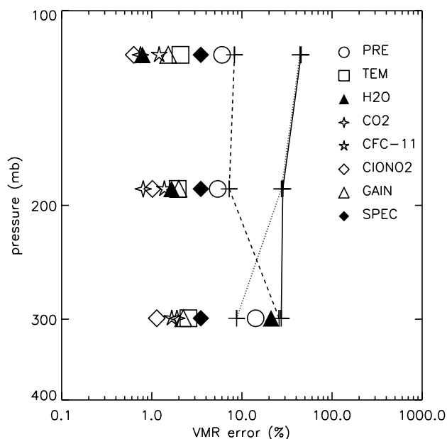
Fig. 2. Mean global error budget for HCFC-22 vmr retrievals. The solid black line represents the total error on a single retrieval. The random (dotted) and systematic (dashed) component of the error are also shown. Systematic errors are dominated by pressure (“PRE”), HCFC-22 spectroscopy (“SPEC”), gain, temperature (“TEM”), ClONO 2 and CFC-11 uncertainties.
