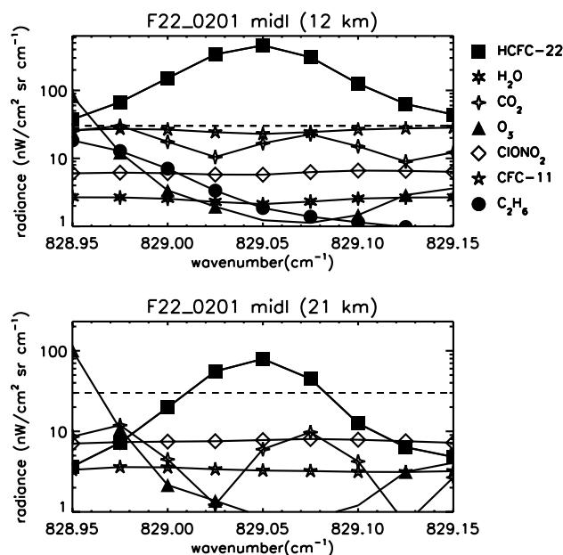
Fig. 1. Plot of modelled radiance contributions from the dominant radiatively active gases in the 828.95 to 829.15 \text{cm}^{-1} range in the mid-latitudes (20 to 65°). The black dotted line represents a “typical” MIPAS-E in flight noise equivalent spectral radiance (NESR) of 30 \text{nW}/(\text{cm}^2 \text{sr cm}^{-1}) , for band A, based on the findings of Klei-ert et al. (2007).
