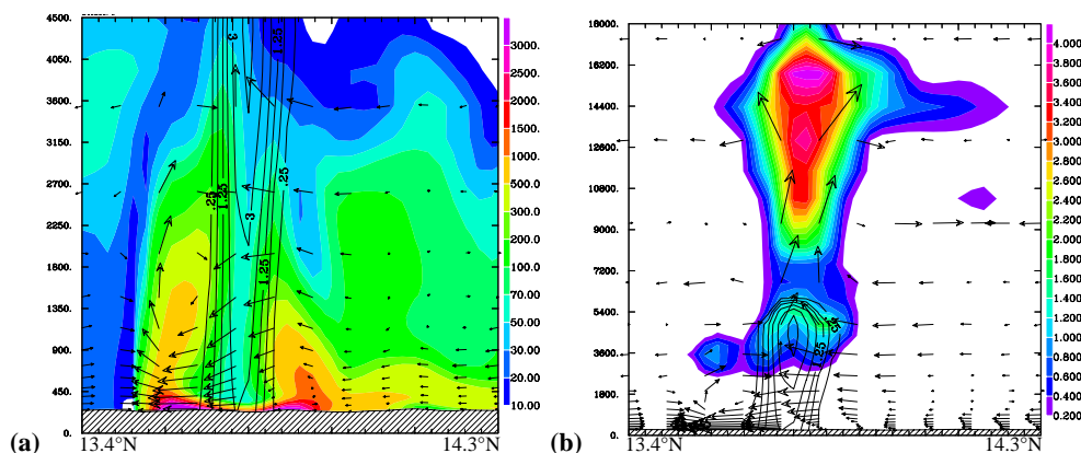
Fig. 15. Meridional cross section of the convective system (see location in Fig. 14) on 1 July 2006, 19:00 UTC. (a) Colored areas represent the mixing ratio for cloud and ice ( \text{g kg}^{-1} ) and the isolines correspond to the mixing ratio for rain ( \text{g kg}^{-1} ). (b) Colored areas represent the dust concentration ( \mu\text{g m}^{-3} ) and the isolines correspond to the mixing ratio for rain ( \text{g kg}^{-1} ). Vertical scales are not the same.
