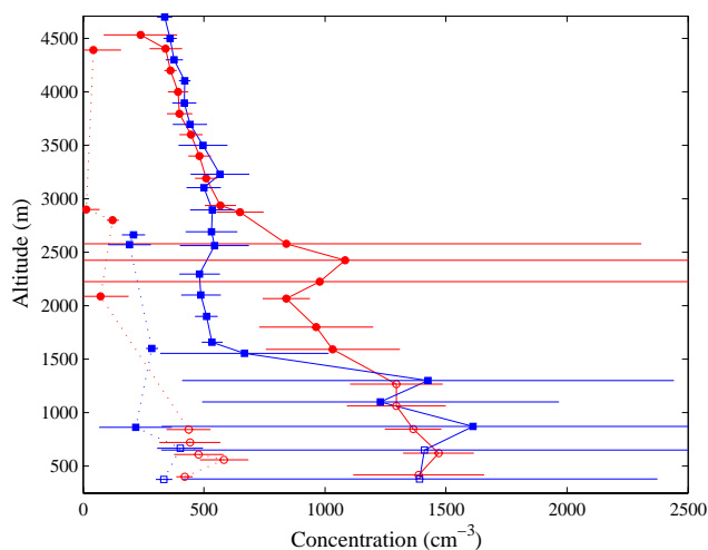
Fig. 5. CN total concentration (solid line) and \text{CCN}_{0.6} concentration (dotted line) as a function of altitude. Red dots are data collected on 1 July 2006, and blue squares are for those collected on 2 July 2006. The open symbols represent the data in the BL and solid symbols represent the data in the SAL. Horizontal bars correspond to the error bar of the average concentrations ( \pm 1\sigma ).
