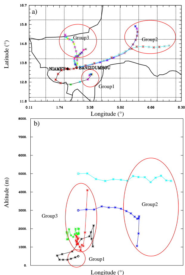
Fig. 13. Backtrajectories ending over Banizoumbou on 2 July 2006, 07:00 UTC. Timestep: 1 h. (a) Horizontal projection. (b) West-east vertical projection.
