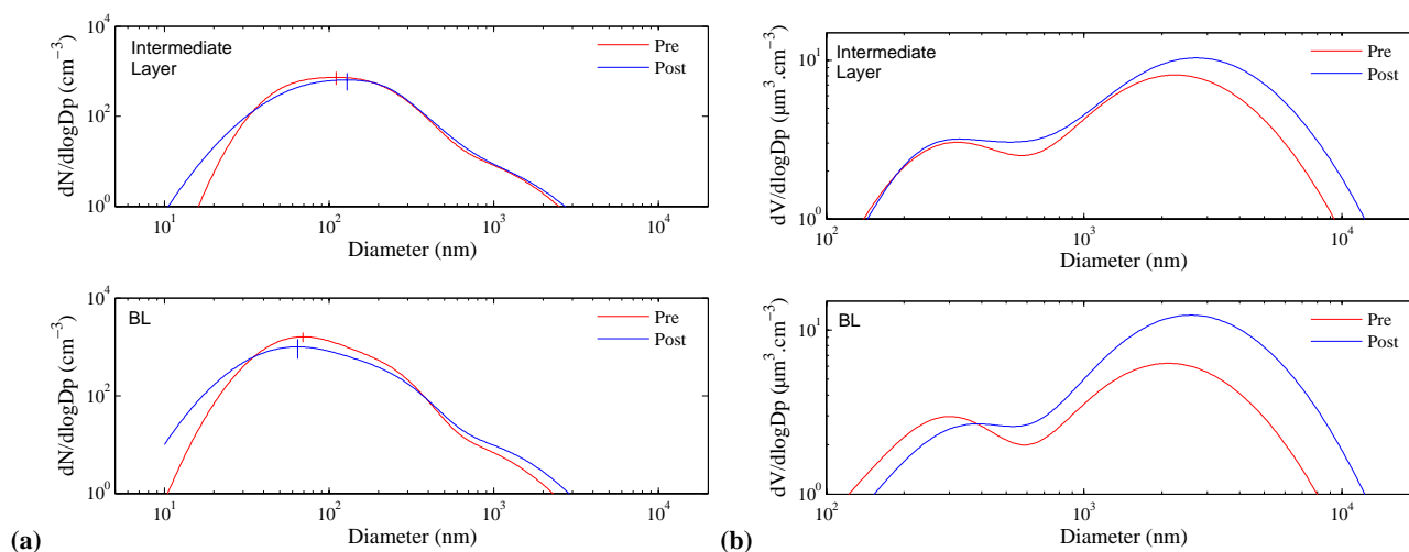
Fig. 7. (a) Average number-size distribution and (b) volume-size distribution observed by the SMPS and the OPS during 1 (red) and 2 (blue) July 2006, in the intermediate layer (top) and in the BL (bottom).
