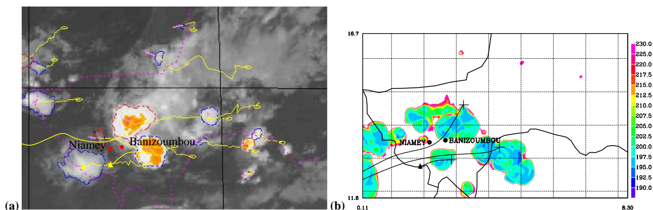
Fig. 9. Comparison between (a) observed satellite image on 2 July 2006, at 00:00 UTC (source: aoc.amma-international.org/observation/mcstracking ) and (b) modeled brightness temperature on 1 July 2006 at 19:00 UTC. On (a) (resp. b), the crosses correspond to the MCS initialisation, the yellow (black) lines correspond to the MCS trajectories and the yellow (black) triangles correspond to the MCS disappearance.
