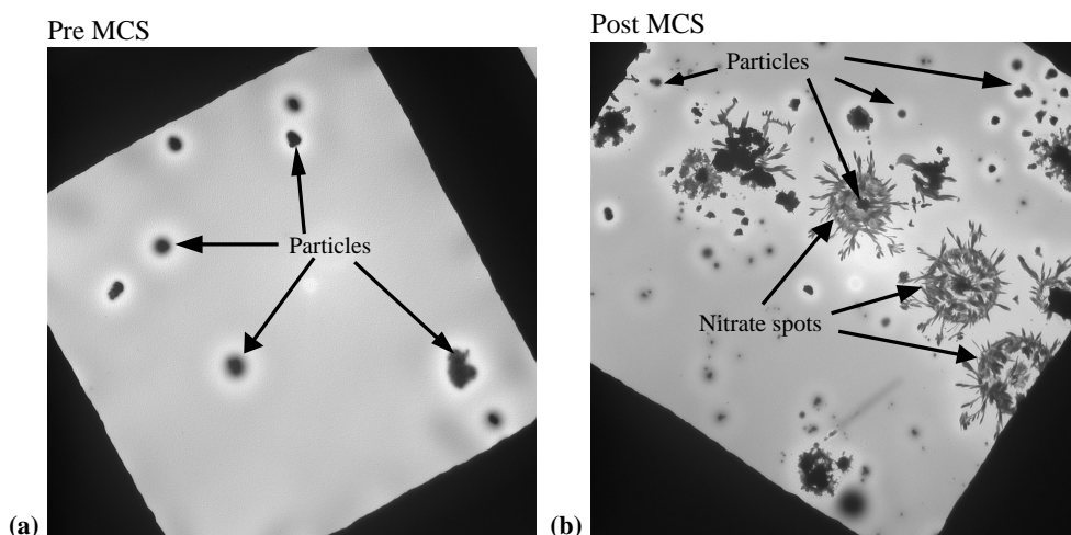
Fig. 8. SEM photographs showing particles collected on the first impactor stage ( D_p > 1.6 \mu\text{m} ) on a nitron filter (a) sampling at 2790 m during 1 July 2006 flight and (b) sampling at 3090 m during 2 July 2006 flight.
