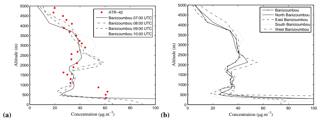
Fig. 11. (a) Comparison of modeled (lines) and observed (dots) vertical profiles of aerosol ( D_p < 2.5 \mu\text{m} ) mass concentration over Banizoumbou. The measurements were made during the ATR-42 flight on 2 July 2006, between 11:00 UTC and 14:00 UTC. (b) Comparison of modeled vertical profile of the aerosol mass concentration over Banizoumbou, 0.5^\circ north of Banizoumbou, 0.5^\circ south of Banizoumbou, 0.5^\circ east of Banizoumbou and 0.5^\circ west of Banizoumbou on 2 July 2006, at 08:00 UTC (12 h after the MCS passage).
