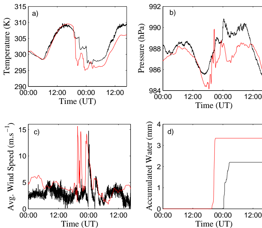
Fig. 10. Modeled (red line) and observed (black line) parameters (a) Temperature ( ^{\circ}\text{K} ) (b) Pressure (hPa) (c) Averaged wind speed ( \text{m s}^{-1} ) (d) Accumulated water (mm), from 1 July, 00:00 UTC to 2 July 18:00 UTC.
