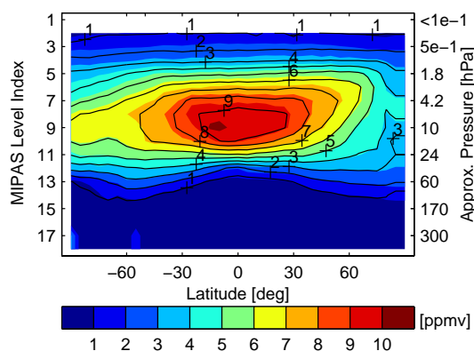
Fig. 1. Zonal mean of O 3 (ppmv) from MIPAS (isocontours) and BASCOE (isolines) on 6 October 2003 and averaged on a 5° latitude grid. The left-hand side vertical axis is the MIPAS vertical level index (1 highest, 17 lowest).
