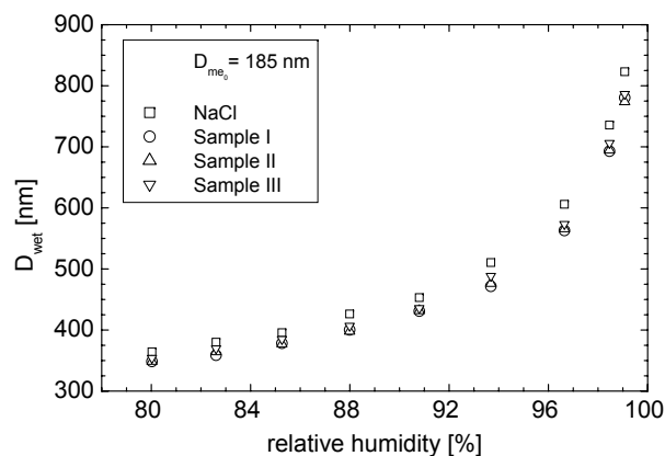
Fig. 4. Hygroscopic growth of sea-salt particles of the three different samples at different values of RH in comparison to pure NaCl. For clarity, error bars are not shown.
