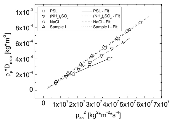
Fig. A2. The product \rho_p D_{mob} is plotted against p_{50}^2 for the PSL, NaCl, (\text{NH}_4)_2\text{SO}_4 and sea-salt (sample I) particles, to determine the shape factor of the (\text{NH}_4)_2\text{SO}_4 and the different sea-salt particles.
