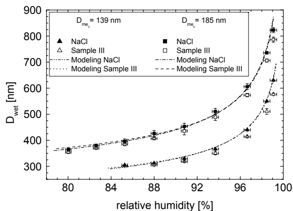
Fig. 3. Hygroscopic growth of the sea-salt particles of sample III at different values of RH compared to that of pure NaCl. For comparison, theoretical curves for sea-salt sample III and NaCl are presented, too.
