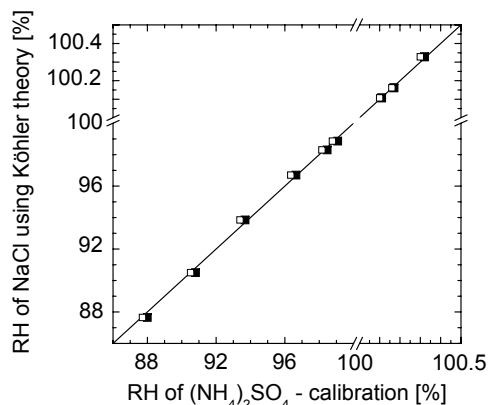
Fig. B1. RHs as determined from the hygroscopic growth of NaCl particles with D_{\text{me0}}=185 nm are plotted versus RHs resulting from the calibration with ammonium sulfate particles ( D_{\text{mob}}=200 nm) assuming a shape factor of 1.00 (open squares) and a shape factor of 1.04 (filled squares), respectively. Additionally, the NaCl data points, received from the activation measurements ( \text{RH}>100\% ) are plotted.
