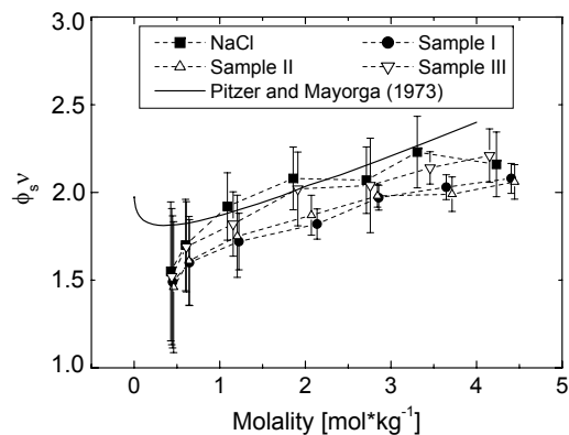
Fig. 7. \phi_s \nu derived from the measured hygroscopic growth for NaCl and the three sea-salt samples in comparison to values for NaCl as given in literature (Pitzer and Mayorga, 1973).
