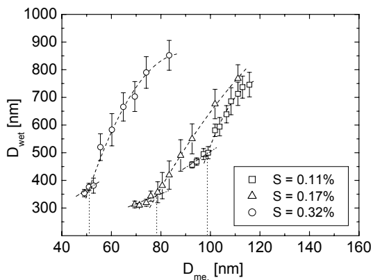
Fig. 5. Activation curves of the sea-salt particles of sample III at three different supersaturations. The intercept point of the polynomial curve and the straight line indicates D_{\text{crit}} .
