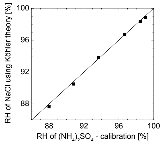
Fig. 2. RHs as determined from the hygroscopic growth of NaCl particles with D_{\text{me}_0}=185 nm are plotted versus RHs resulting from the calibration with ammonium sulfate particles with D_{\text{me}_0}=192 nm.
