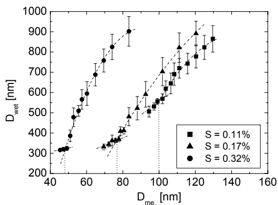
Fig. 6. Activation curves of the NaCl particles at three different supersaturations. The intercept point of the polynomial curve and the straight line indicates D_{\text{crit}} .
