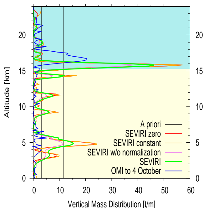
Fig. 7. Sensitivity experiments with the inversion algorithm: SEVIRI (green line) is the same result as shown in Fig. 6; SEVIRI constant (orange line) is using a flat a priori profile (shown by the thick black line) and uncertainty (thin black line); SEVIRI zero is using a zero emission a priori (red line) with the same flat uncertainty range as in the constant a priori scenario; SEVIRI w/o normalization (violet line) is using the data without normalization of the total mass to the OMI total mass, and OMI to 4 October (blue line) is using OMI data until 4 October 2007.
