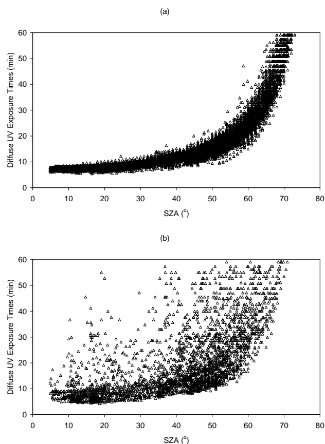
Fig. 3. Times for exposure to 1/3 MED of diffuse UV for cloud cover of 0 to 80% (a) and 85 to 100% (b).
