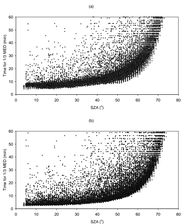
Fig. 2. The times required for an exposure of 1/3 MED due to diffuse UV ery (a) and global UV ery (b) as a function of SAZ for all sky conditions during 2003.
