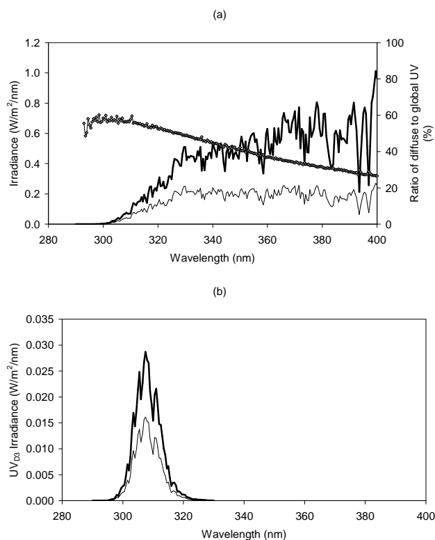
Fig. 1. Diffuse (light line) and global (heavy line) spectral UV irradiances taken on 17 August 2005 at approximately 11:00 EST and the spectral ratio of diffuse to global UV (a); and global and diffuse spectral irradiances from Fig. 1a weighted with the pre-vitamin D 3 action spectrum (CIE, 2006) (b).
