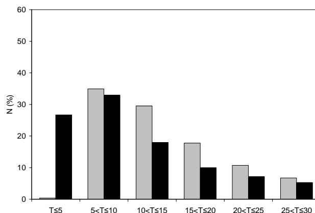
Fig. 4. The percentage of instances when the time required for an exposure of 1/3 MED due to diffuse (grey bar) and global (black bar) UV_{ery} falls within a certain time range (provided in units of minutes).
