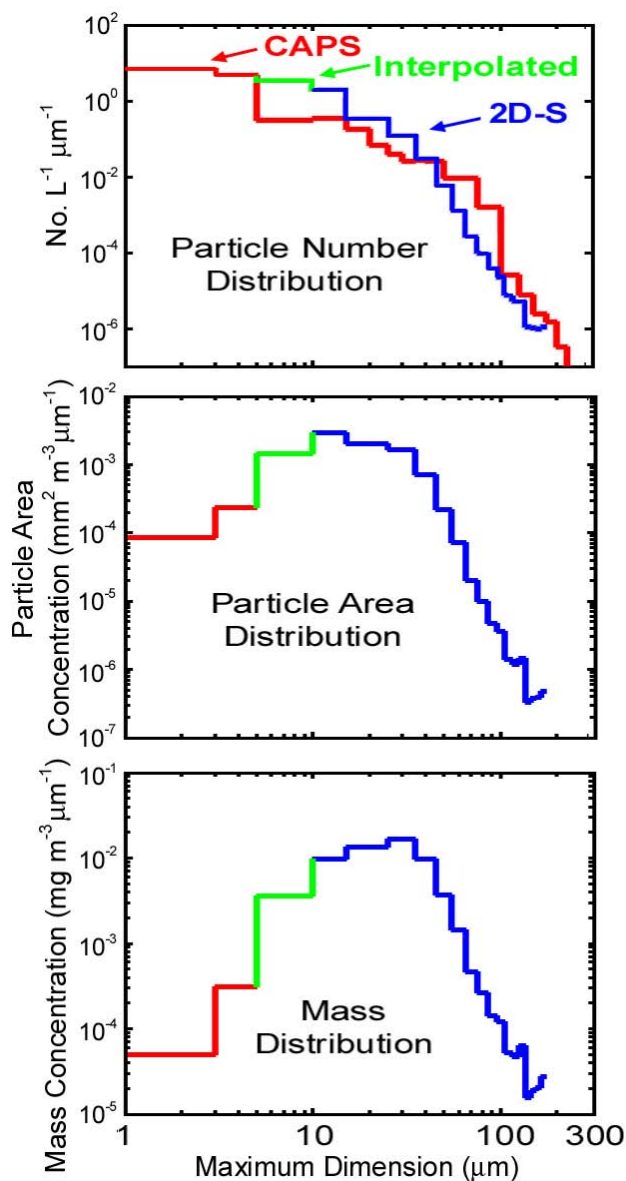
Fig. 8. PSD's of (top) number concentration, (middle) area and (bottom) mass based on \sim 1800 km of WB-57F 2D-S and CAPS measurements collected in SVC. Green trace is interpolated between 5 \mu\text{m} CAS and 10 \mu\text{m} 2D-S size bins.
