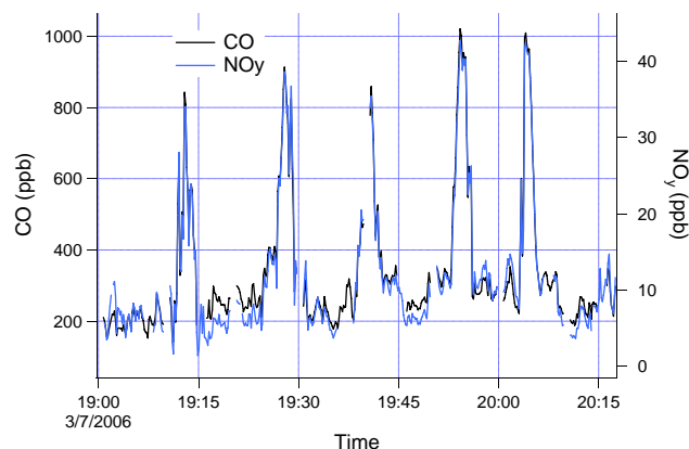
Fig. 3. Time series in UTC for CO and \text{NO}_y on flight 307a containing 5 passes through the urban plume encountered on Legs 4 and 5. Proportionality between CO and \text{NO}_y causes CO trace to be largely hidden by \text{NO}_y trace during plume passages.
