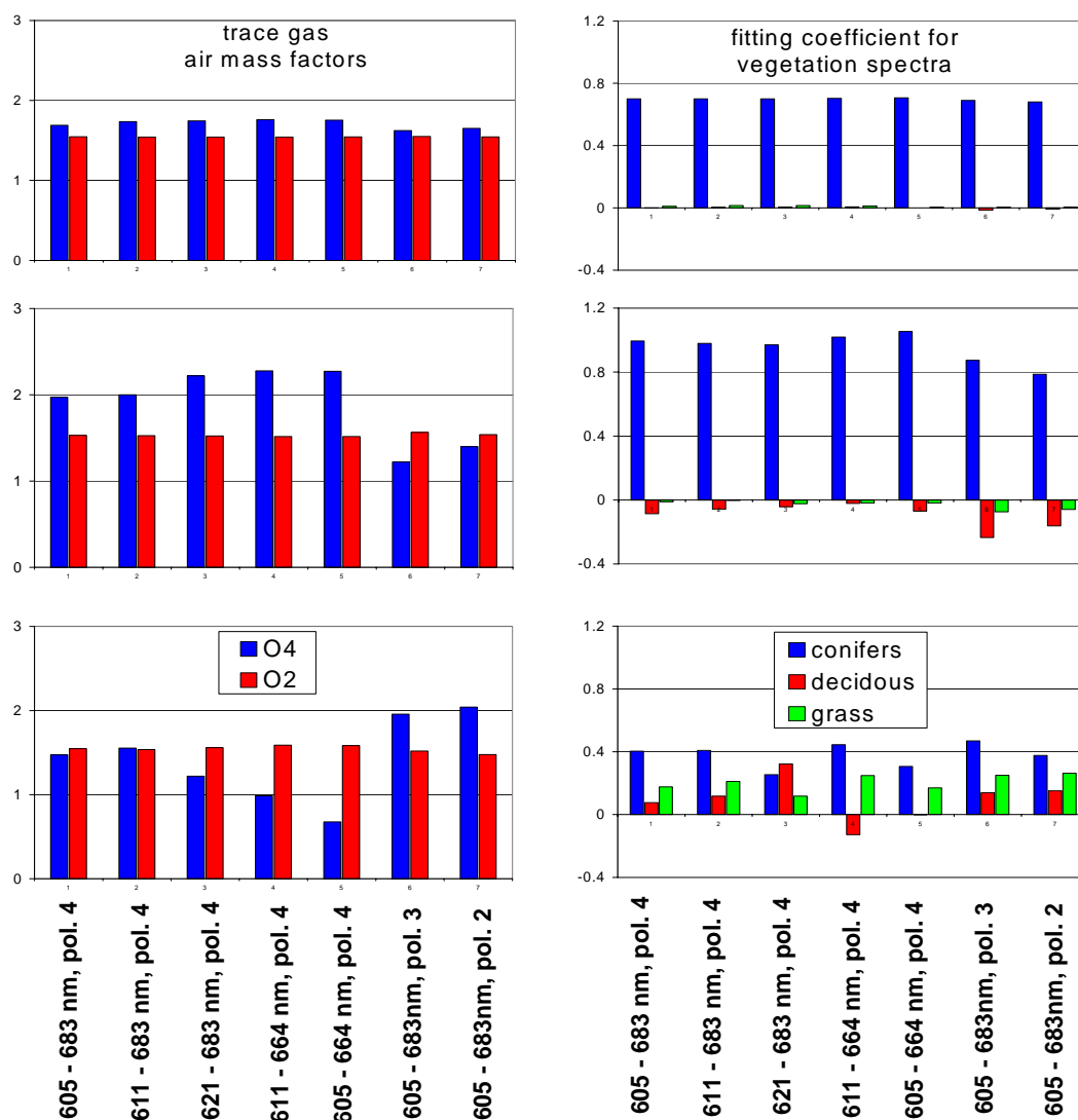
Fig. 6. Results for the DOAS analysis of modelled spectra using the original vegetation spectra (top), using vegetation spectra convolved by a Gaussian function of 4.6 nm FWHM (middle), or using vegetation spectra shifted by -1 nm (bottom). The spectra were modelled for a SZA: 10^\circ , without aerosols, and for a conifers spectrum as albedo. The different results in the individual graphs are retrieved for different fitting parameters. If the original vegetation spectra are used in the DOAS retrieval, the DOAS results hardly depend on the fitting parameters (top). They also fit the expected values (air mass factor of slightly lower than 2 for the trace gas absorptions; fitting coefficient of about 0.7 for the conifer spectrum, 0 for the other vegetation spectra). If smoothed or shifted vegetation spectra are used, the results differ from the expected values and also strongly depend on the fitting parameters.
