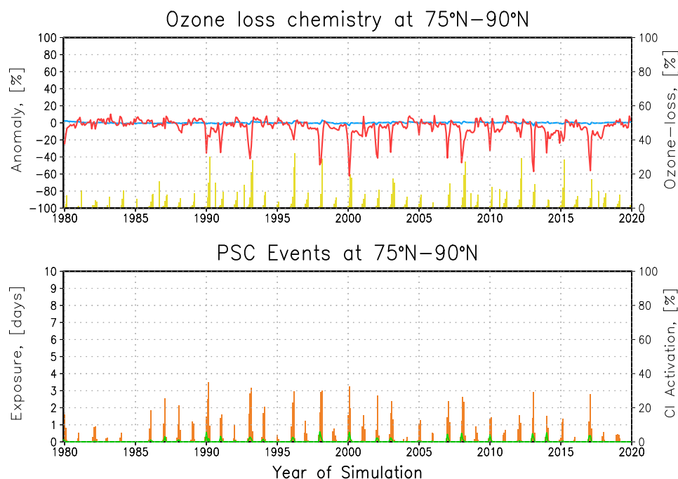
Fig. 6. Simulated evolutions for 1980–2019 of main constituents affecting ozone within 75^{\circ} N, and between 146 and 31 hPa. In the upper frame the percentage anomalies in total nitrogen is shown by the red line and in water vapour by the blue line. The relative difference between the passive ozone tracer and regular model ozone by yellow bars. In the lower frame the chlorine activation is shown by orange bars, the PSC type-I tracer is given by the green line and the PSC type-II tracer by the black line.
