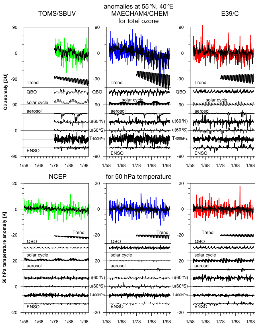
Fig. 3. Same as Fig. 2, but for the grid point nearest to 55^{\circ} N, 40^{\circ} E.
