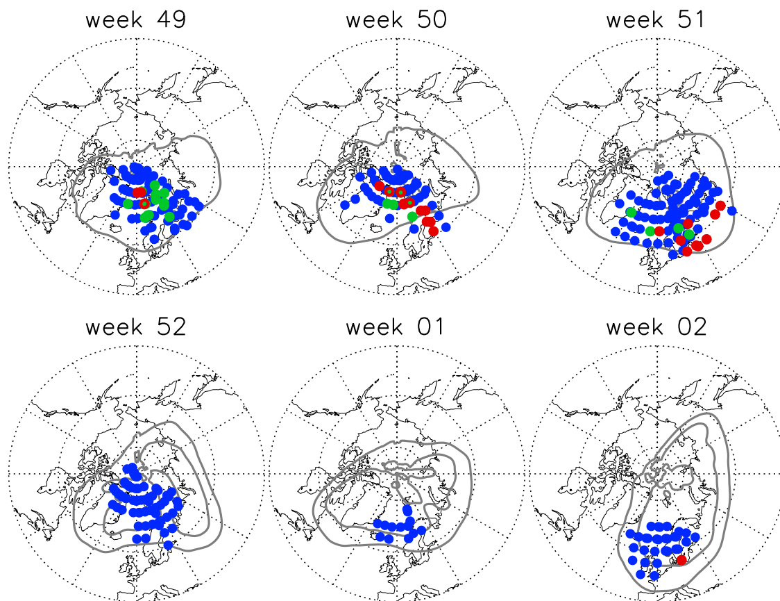
Fig. 9. Temporal evolution of the PSC events with (most likely NAT /red) and without a strong radiation enhancement at 820\text{ cm}^{-1} (presumably STS and/or mixed type clouds/in blue) shown for the last four weeks of 2002 (week 49–52) and first two weeks in January 2003 (week 1–2) in the latitude range 40^\circ to 90^\circ N. Green dots highlight events with CI < 1.5 which refers to events with large optical thickness. The grey contours represent the 60 and 80 PVU contour for midweek conditions at 550 K.
