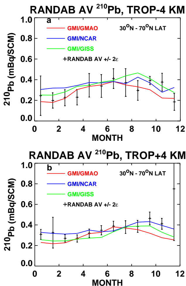
Fig. 11. Comparison of observed and simulated midlatitude average seasonal cycle of ^{210}\text{Pb} in the: (a) tropopause -4 km region, and (b) tropopause +4 km region. Observed distributions are calculated by averaging data from the US Environmental Measurement Laboratory RANDAB database between 30^\circ – 70^\circ by month. Tropopause height estimates are obtained as described in caption for Fig. 10. Simulated output is treated as described in caption for Fig. 10.
