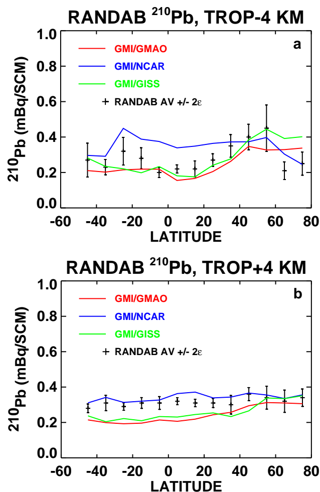
Fig. 10. Comparison of observed and simulated meridional distributions of ^{210}\text{Pb} in the: (a) tropopause -4 \text{ km} region, and (b) tropopause +4 \text{ km} region. Observed distributions are calculated by averaging data from the US Environmental Measurement Laboratory RANDAB database into 10^\circ bins centered at -45^\circ , -35^\circ , ..., 75^\circ . Tropopause height estimates for the RANDAB data are not part of the climatology. These were determined by calculating the thermal tropopause height at the location and time of the observations using the NCEP 50-year reanalysis (Kistler et al., 2001). Error bars represent \pm 2 times the standard error of the averages. Simulated distributions are obtained by sampling model at observation locations and treating the sampled output in the same manner as the observations.
