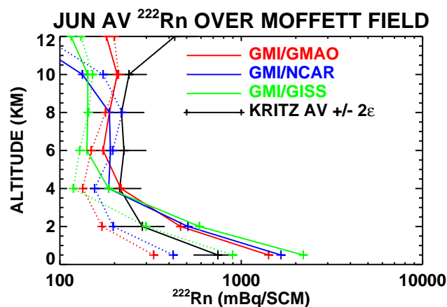
Fig. 6. Comparison of GMI model simulations of vertical 222 Rn profiles with profiles constructed from observations taken over Moffett Field, CA in June (Kritz et al., 1998). Black solid line shows June average profile from observations. Error bars represent ±2 times the standard error of the averages. Solid colored lines represent model profiles over Moffett field. Dotted colored lines are profiles from 5° longitude west of the Moffett field profiles to indicate longitudinal gradients in 222 Rn.
