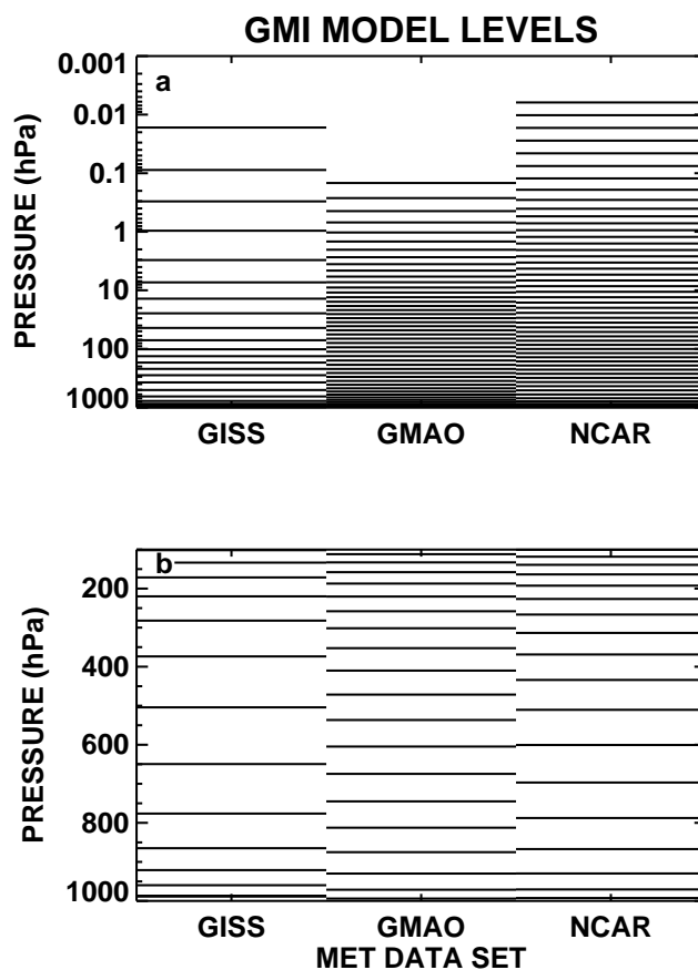
Fig. 1. Spacing of vertical levels in the three GMI simulations, assuming a surface pressure of 1000 hPa. (a) shows the model level midpoint values over the entire vertical ranges of the meteorological data. (b) shows the spacing up to 100 hPa.
