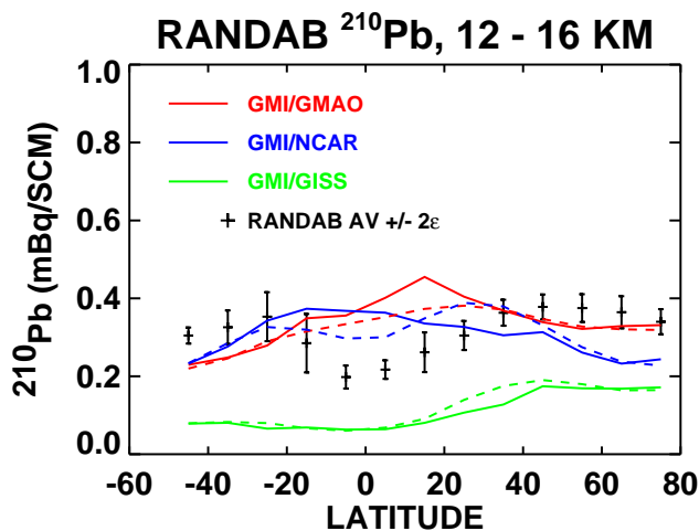
Fig. 14. Same as Fig. 9a, except that the model meridional distributions are from simulations in which the convective transport and scavenging operator was not called.
