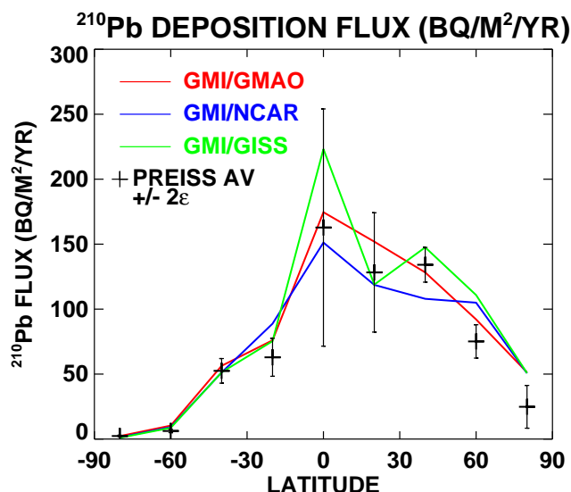
Fig. 2. Meridional distribution of annually averaged ^{210}\text{Pb} deposition flux in the GMI model simulations compared to observations, in \text{Bq m}^{-2} \text{ yr}^{-1} . Observations were grouped into 20^\circ latitude bins and averaged. Error bars represent \pm 2 times the standard error of the average values. Model values were obtained by interpolating the gridded output to each site location, then averaging model output in same manner as observations.
