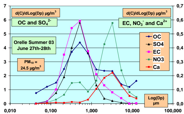
Fig. 14. Daily size distributions of the concentrations of OC, EC, sulfate, nitrate, and calcium obtained in Orelle (rural site in the Maurienne Valley) on 27 June 2003.
