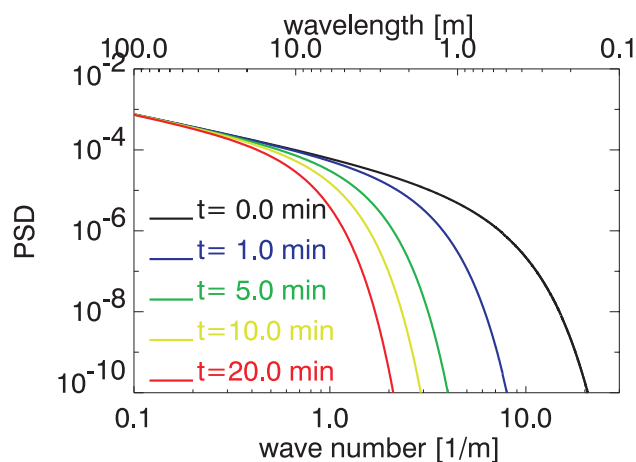
Fig. 6. Power spectra of tracer variance according to Eq. (3) and (7) for a turbulent energy dissipation rate \epsilon=0.1 \text{ m}^2/\text{s}^3 , kinematic viscosity \nu=1.5 \text{ m}^2/\text{s} , an aerosol radius r_A=10 \text{ nm} , and different times after active neutral air turbulence stopped (color coded).
