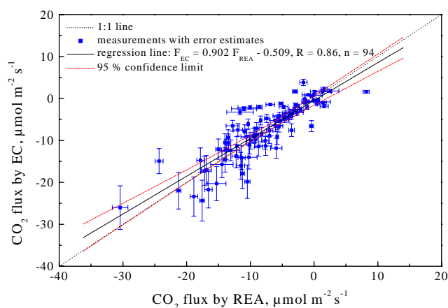
Fig. 4. Intercomparison of the \text{CO}_2 fluxes obtained by REA with those from EC measurements.
