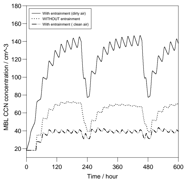
Fig. 6. CCN concentration with entrainment (solid line), without entrainment (dotted line), and with entrainment of clean air from FT (dashed line). The mean values for these simulation were 126 , 63 and 39 \text{ cm}^{-3} , respectively.
