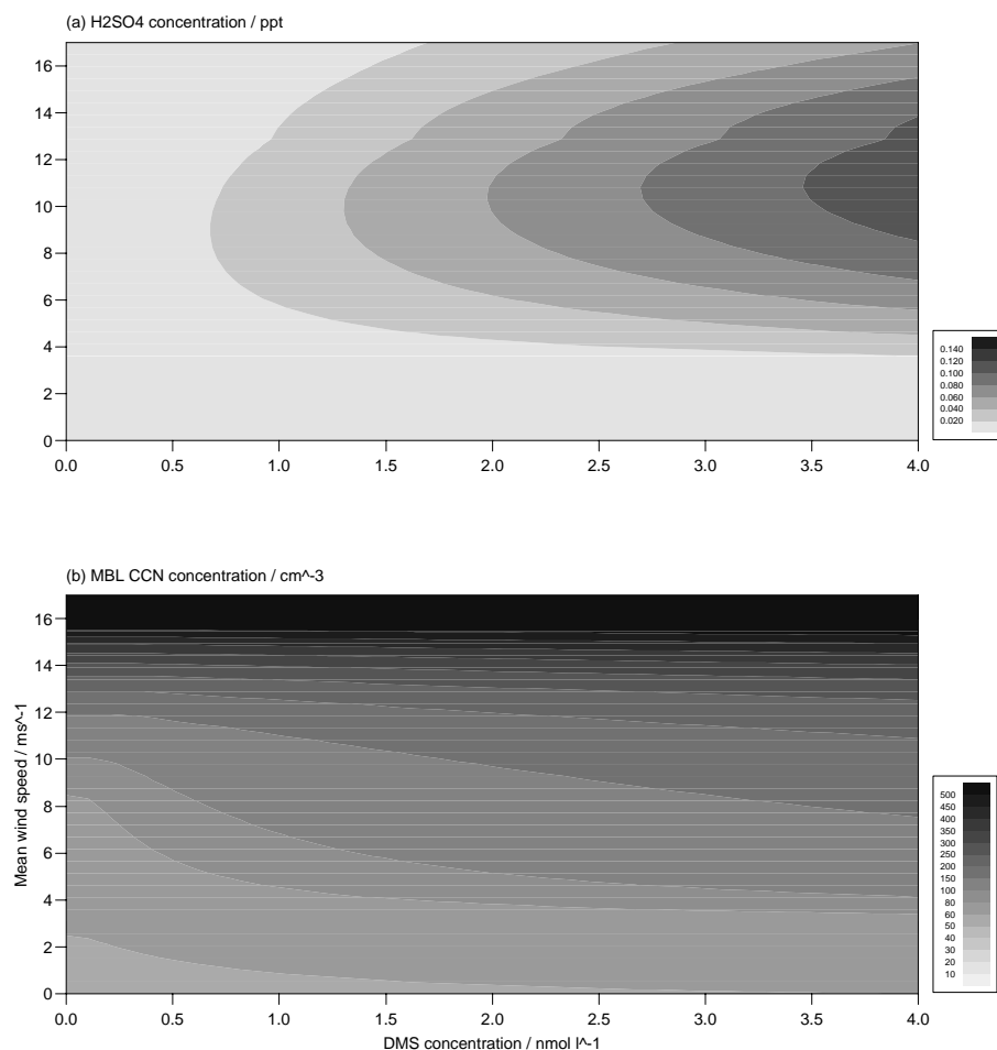
Fig. 7. Predicted distributions of (a) gaseous H 2 SO 4 (ppt), and (b) MBL CCN (cm -3 ) concentration. This simulation used the default parameters except for seawater DMS concentration and mean wind speeds.
