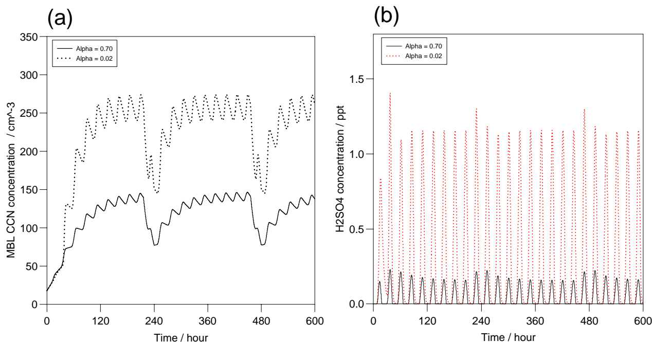
Fig. 5. (a) MBL CCN and (b) \text{H}_2\text{SO}_4 variation with \alpha = 0.02 and \alpha = 0.70 . The entrainment terms in the reactions were included in this case. The averaged concentrations for MBL CCN and (\text{H}_2\text{SO}_4)_g were 238 \text{ cm}^{-3} and 0.34 \text{ ppt} , when an accommodation coefficient of 0.02 was used instead of 0.70 .
