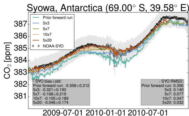
Figure 6. Time series of measured and modeled \text{CO}_2 concentrations at Syowa Station, Antarctica, for CarbonTracker runs with different lengths of the assimilation time window. The baseline run uses an assimilation window of 5 \times 7 days. Color coding of shorter and longer assimilation windows follows the legend (lag \times cycle in days).
