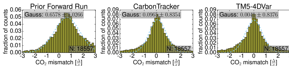
Figure 4. Histograms of the mismatch between measured and modeled \text{CO}_2 concentrations for all non-assimilated samples using prior fluxes, CarbonTracker optimized fluxes and TM5-4DVar optimized fluxes. The histograms show residuals for one year (3 April 2009 to 2 April 2010) which are normalized by the estimated representativeness error. The line on top of the histograms is a fit of a Gauss function to the histogram. The parameters in the top left show the bias and standard deviation of the histogram. The bottom right shows the number of measurements which were accumulated into the histogram.
