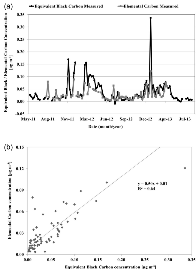
Figure 1. (a) Weekly measured EBC and EC concentrations in \mu\text{g m}^{-3} from May 2011 to August 2013 at VRS (Station Nord), North Greenland. Both EBC and EC show the same seasonal variation with maximum concentrations in winter and spring and minimum concentrations in summer, (b) scatter plot of measured EC and EBC concentrations (the slope obtained by orthogonal regression is y = 0.50 showing a correlation coefficient of R^2 = 0.64 ).
