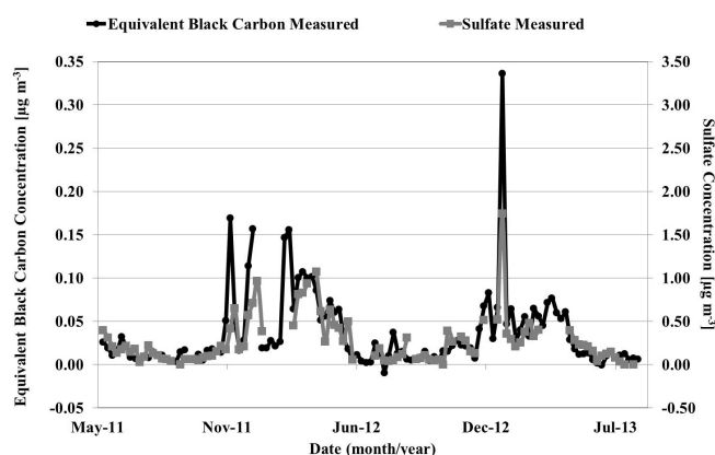
Figure 2. Weekly measured EBC and sulfate concentrations in \mu\text{g m}^{-3} from May 2011 to August 2013 at VRS (Station Nord), North Greenland. Here, EBC and sulfate concentrations exhibit very similar patterns with maximum concentrations in winter and spring compared to minimum concentrations in summer.
