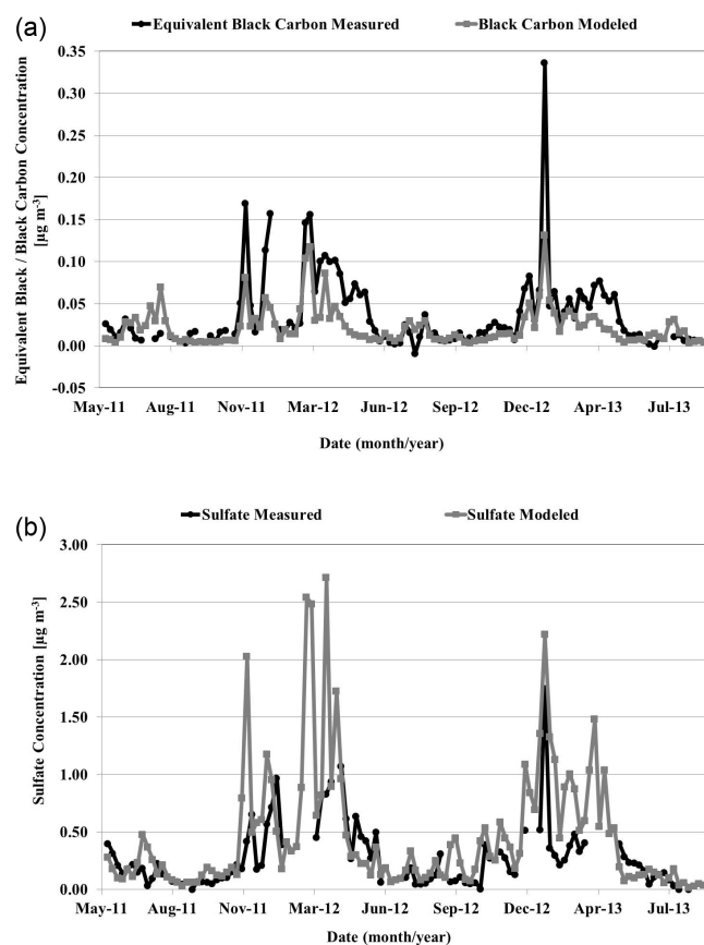
Figure 3. Comparison of measurement and model results from DEHM for (a) EBC/BC and (b) sulfate concentrations at VRS (Station Nord), North Greenland, during the time period from May 2011 to August 2013.
