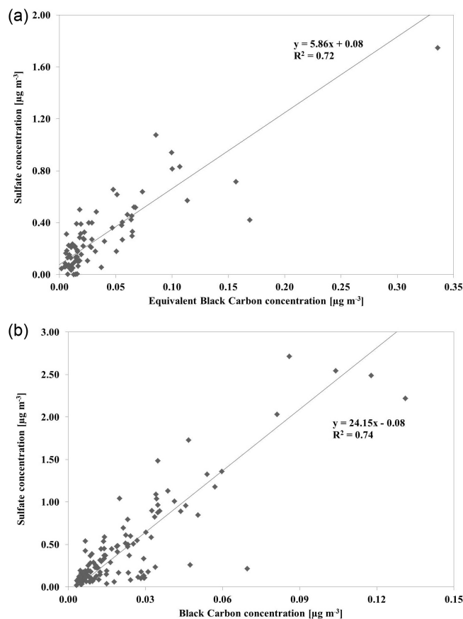
Figure 4. Scatter plot of EBC/BC and sulfate concentrations based on (a) measurement results (the slope obtained by orthogonal regression between sulfate and EBC is y = 5.86 showing a correlation coefficient of R^2 = 0.72 ) and (b) model results (the slope obtained by orthogonal regression between sulfate and BC is y = 24.15 showing a correlation coefficient of R^2 = 0.74 ) during May 2011 to August 2013 at VRS (Station Nord), North Greenland.
