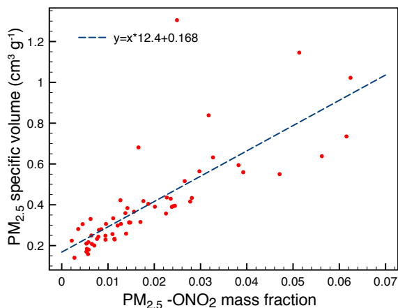
Figure 4. Correlation of specific volume (inverse density) to the mass fraction of the aerosol organic nitrate for \text{PM}_{2.5} size range ( R^2 = 0.6 ).
