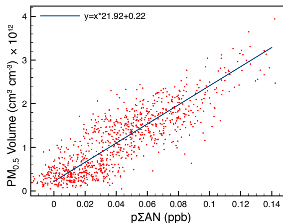
Figure 3. Correlation of \text{PM}_{0.5} volume measured by SMPS to particulate organic nitrate concentration ( R^2 = 0.72 ).
