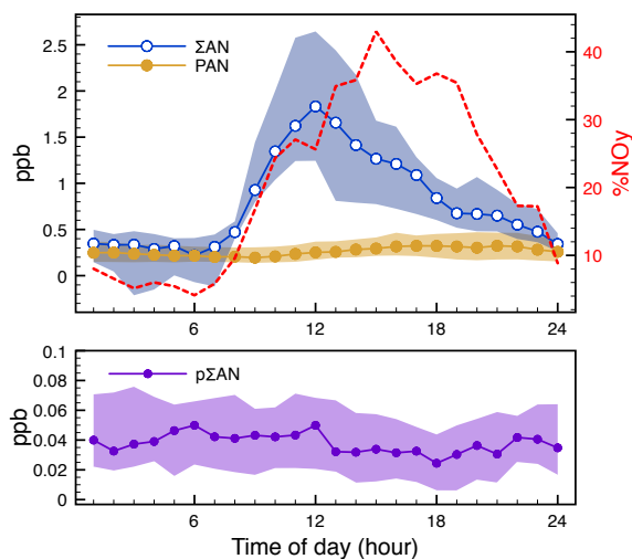
Figure 2. Average mixing ratios of total alkyl nitrate ( \Sigma\text{AN} , blue), PAN (yellow), (\Sigma\text{AN}/\text{NO}_y) \times 100\% (red dashed) and p\Sigma\text{AN} (purple) vs. time of day. Interquartile range is shaded.
