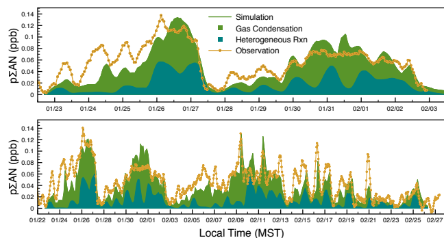
Figure 6. Time series of predicted particulate organic nitrate concentration from box model simulation for two accumulation events (top panel) and the campaign period (bottom panel) as stacked areas showing contribution from each of the two mechanisms responsible. The observations are plotted in yellow.
