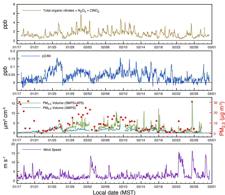
Figure 1. Hourly time series from measurements of total organic nitrates plus \text{N}_2\text{O}_5 and \text{ClNO}_2 , particulate organic nitrate ( p\Sigma\text{AN} ), and total aerosol volume measured by SMPS and APS with filter-sampled \text{PM}_{2.5} mass (red dots, secondary axis) and local wind speed.
