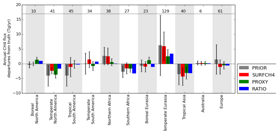
Figure 7. As Fig. 5 for RATIO, PROXY and SURFCH4.
