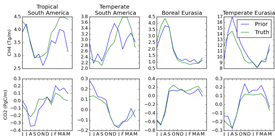
Figure 2. Time series of the true and prior fluxes (per month) integrated over Tropical South America, Temperate South America, Boreal Eurasia and Temperate Eurasia. For CH 4 , we show the total fluxes, and for CO 2 , we show the biosphere fluxes (see Table 1).
