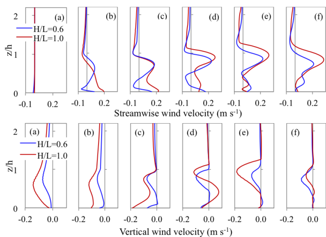
Figure 5. Profiles of streamwise velocity ( u ; \text{m s}^{-1} ; top panel) and vertical velocity ( w ; \text{m s}^{-1} ; bottom panel) for H/L = 0.6 (blue) and H/L = 1.0 (red). The locations of the six sections are labeled as (a)–(f), and their locations with respect to the hill are marked in Fig. 3 with the same letters. Note that wind velocity on the slope surface is not zero because the centers of bottom grid cells in the numerical calculation are not exactly at the surface.
