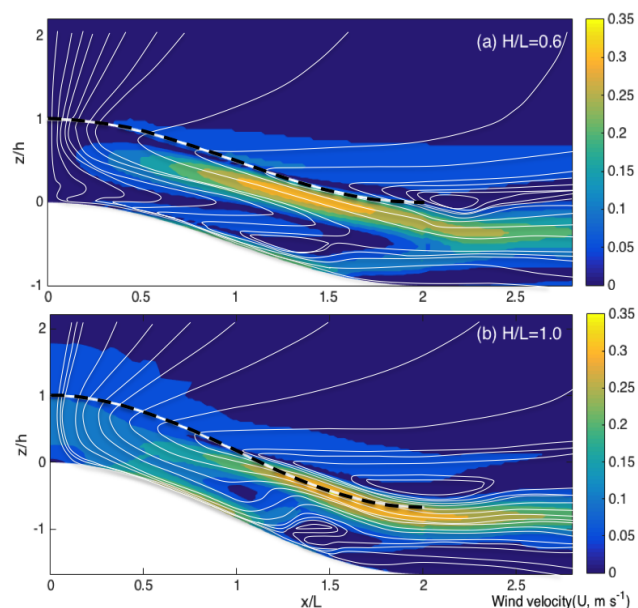
Figure 6. Wind velocity ( U , \text{m s}^{-1} ) on the slopes for (a) H/L = 0.6 and (b) H/L = 1.0 . The white solid lines are streamlines as shown in Fig. 1. The black-white-dashed lines denote the top of the canopy.
