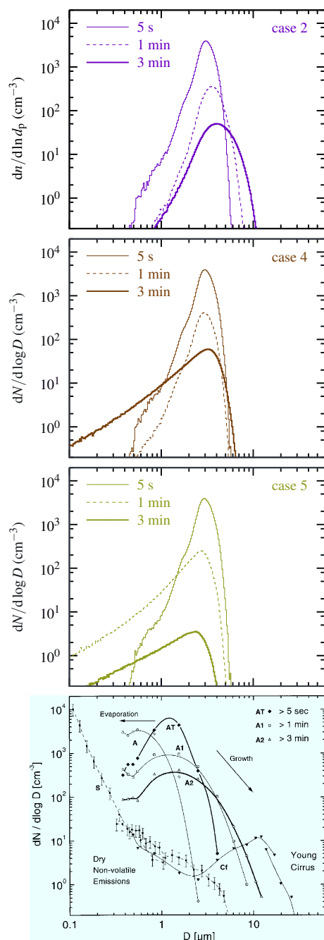
Figure 18. Crystal diameter distributions at 5 s, 1 min, 3 min for the three levels of saturation and measurements from Schröder et al. (2000) (bottom).
