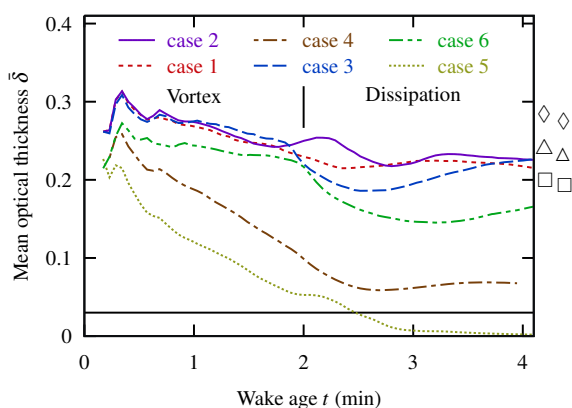
Figure 17. Mean optical thickness. The horizontal black line represent the visibility criterion \bar{\delta} > 0.03 (Kärcher et al., 1996). The mean optical thickness decreases during the vortex regime and stabilizes during the dissipation regime. Its evolution depends mainly on atmospheric temperature, saturation, and, to a lesser extent, turbulence. The symbols on the right of the figure shows the values of the optical thickness for different aircraft and atmospheric situations measured in the CONCERT campaign (Voigt et al., 2011) as reported by Jeßberger et al. (2013).
