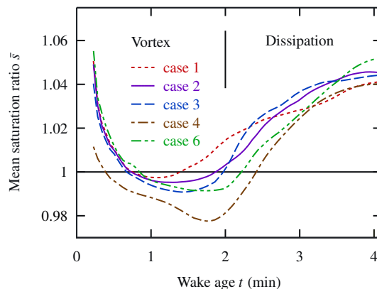
Figure 16. Mean saturation ratio computed as an ensemble average over all ice particles. The contrails are slightly subsaturated during the initial vortex descent between 1 and 2 min and supersaturated in the dissipation phase after 2 min.
