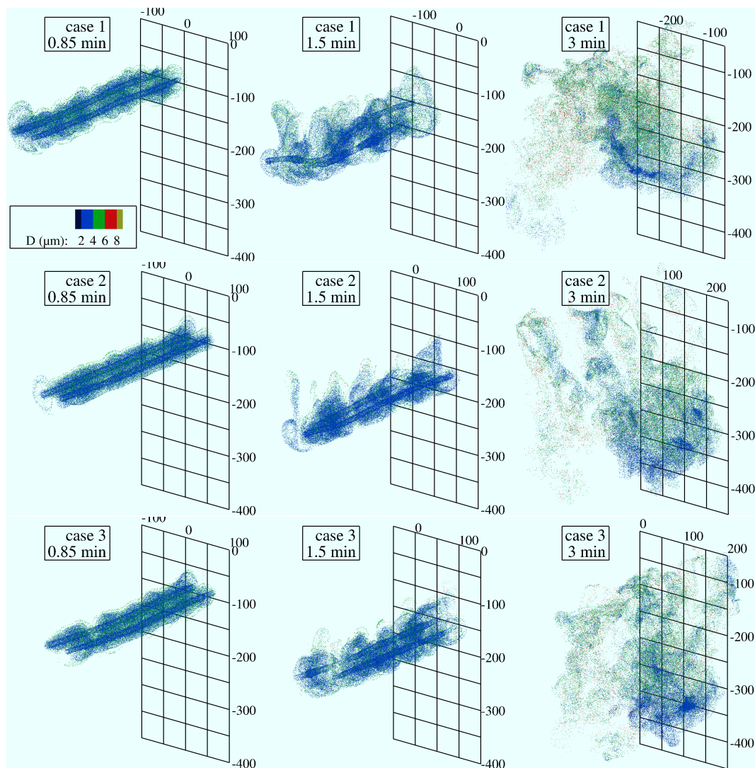
Figure 9. Snapshots of ice crystals spatial distribution for cases 1, 2, and 3. Crystals are colored with diameters. The figure shows the development of the secondary wake at t = 1.5 min and 3 min (center and right panels) and the formation of puffs at t = 3 min (right panels). It can be observed that the size of crystals slightly increases during the instability process of the vortex regime ( t \leq 1.5 min), whereas it increases considerably in the dissipation regime ( t = 3 min) with larger crystals found in the secondary wake. Crystals appear more mixed in the strong atmospheric turbulence case (top panels).
