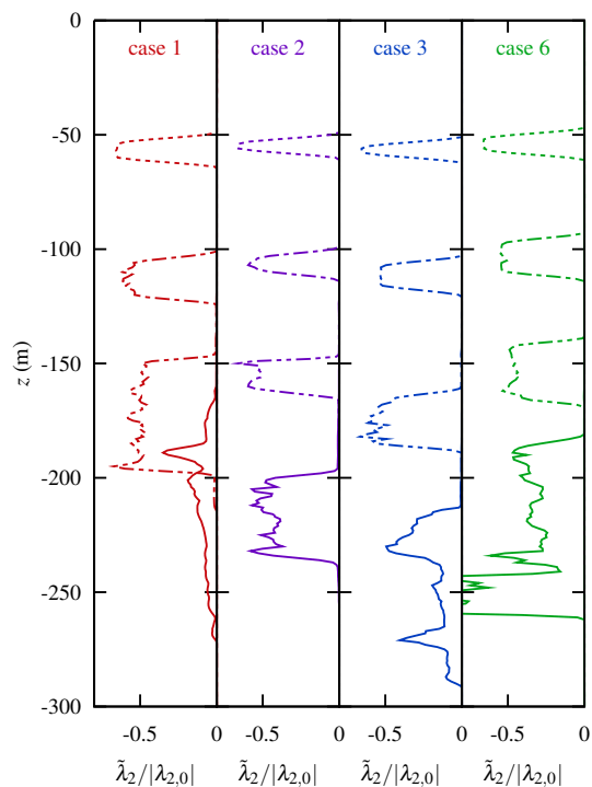
Figure 8. Vertical profiles of \tilde{\lambda}_2/\lambda_{2,0} that is used to track the wake vortices as they move downwards and break up. The four profiles shown for each case correspond to \cdots t = 0.5 min, --- t = 1 min, - \cdot - t = 1.5 min, — t = 2 min.
