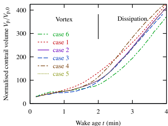
Figure 11. Normalized contrail volume per unit flight distance. Note the increased mixing following the vortex breakup where the exhaust material is released into the atmosphere.
