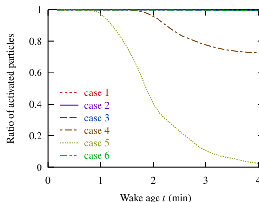
Figure 14. Normalized number of activated particles (fraction of surviving crystals). Adiabatic compression is strong enough in weakly supersaturated atmosphere (case 4) to completely sublimate 30 % of crystals, but it is not able to evaporate any crystals in strongly supersaturated atmosphere.
