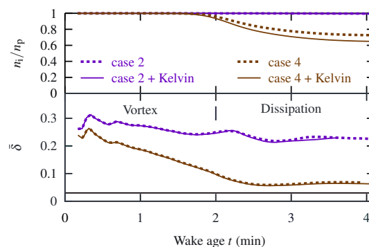
Figure 19. Top panel: normalized number of activated particles (fraction of surviving crystals). Bottom panel: mean optical thickness. Plain lines indicates simulations with the Kelvin effect activated.
