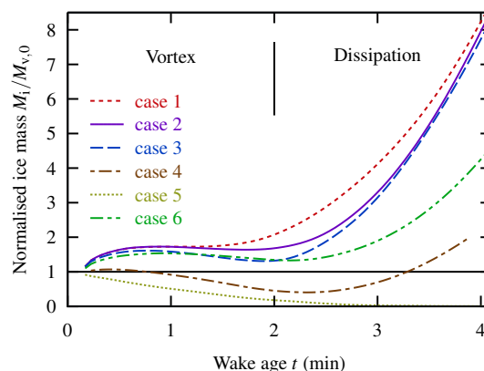
Figure 12. Ice mass per unit flight distance normalized by the mass of emitted water vapor. Adiabatic compression reduces M_i at the end of the vortex regime, and this is particularly effective when the atmosphere is weakly supersaturated (case 4). The breakup of the vortices causes M_i to increase at a rate that depends on atmospheric temperature, saturation, and, to a much lesser extent, turbulence.
