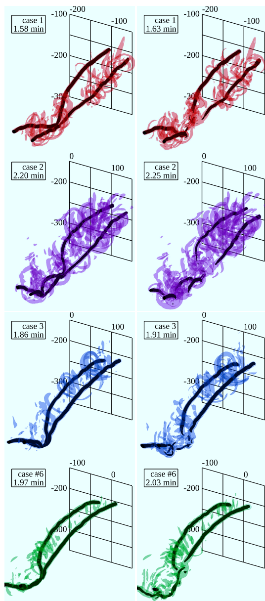
Figure 4. Iso-contours \lambda_2 = \lambda_{2,0}/10 (black) and \lambda_2 = \lambda_{2,0}/1000 (colored) taken immediately before (left panels) and after (right panels) the vortex tubes collide. Black iso-contours represent the wake vortices, while colored iso-contours represent the secondary vortices.
