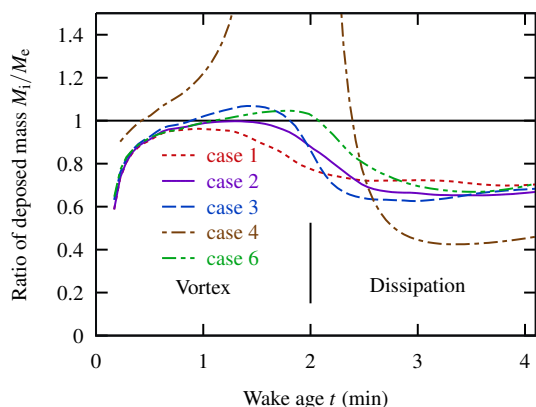
Figure 15. Ratio of deposited mass. In the vortex regime, the contrail is close to equilibrium ( M_i \approx M_e ) only when the atmosphere is strongly supersaturated. In the dissipation regime, the strong mixing between the contrail and ambient air causes a depart from the equilibrium state ( M_i < M_e ).
