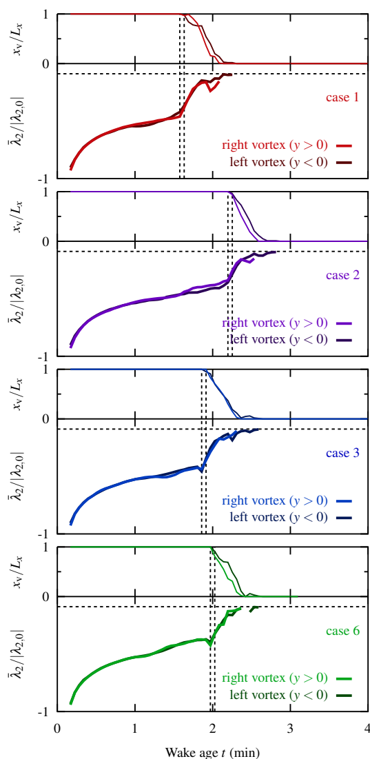
Figure 5. Time histories of vortex length ratios x_v/L_x and \lambda_2/\lambda_{2,0} for cases 1, 2, 3, and 6. The horizontal dashed lines for each case indicate the threshold values \lambda_2 = \lambda_{2,0}/10 that is used to discriminate the wake vortex tubes from the background turbulence. The two vertical dashed lines correspond to the times selected in the iso-contours of Fig. 4 (i.e., immediately before and after the vortex breakup) and define the lifespans of the wake vortices.
