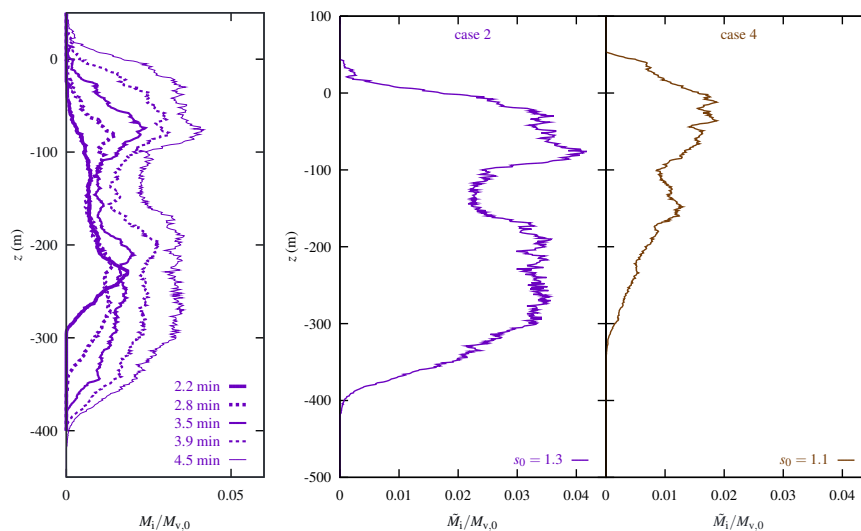
Figure 13. Vertical profiles of normalized mass \tilde{M}_i(z)/M_{v,0} . Left panel: profiles at different wakes ages in the dissipation regime for case 2. Right panel: comparison at t = 4.5 min between case 2 ( s_0 = 1.3 ) and case 4 ( s_0 = 1.1 ).
